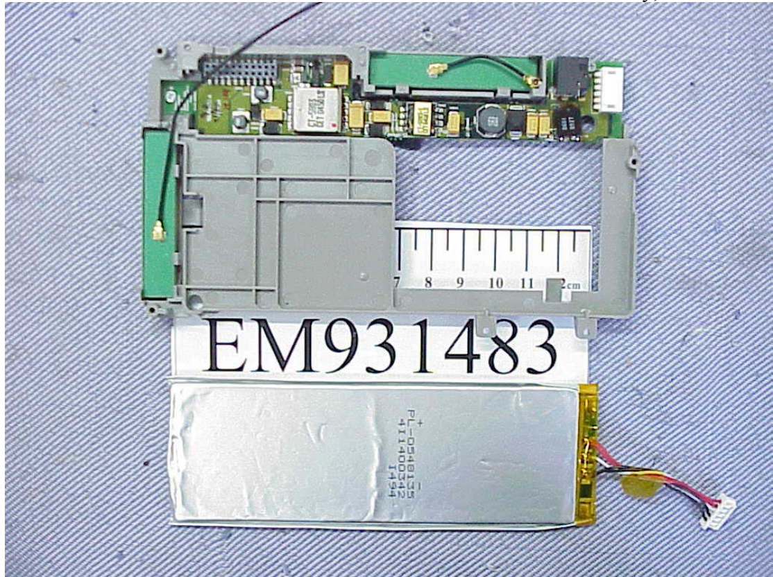
Figure 5 Removed Battery, Internal View
