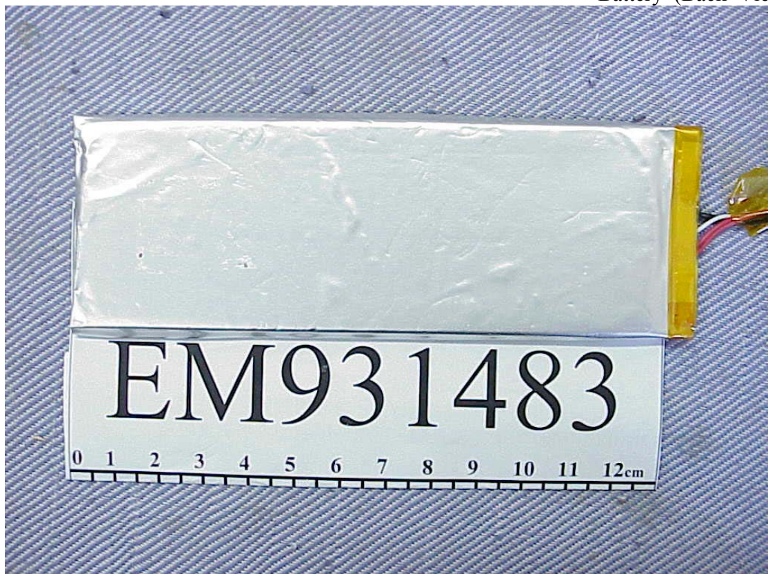
Figure 6 Battery (Back View)
