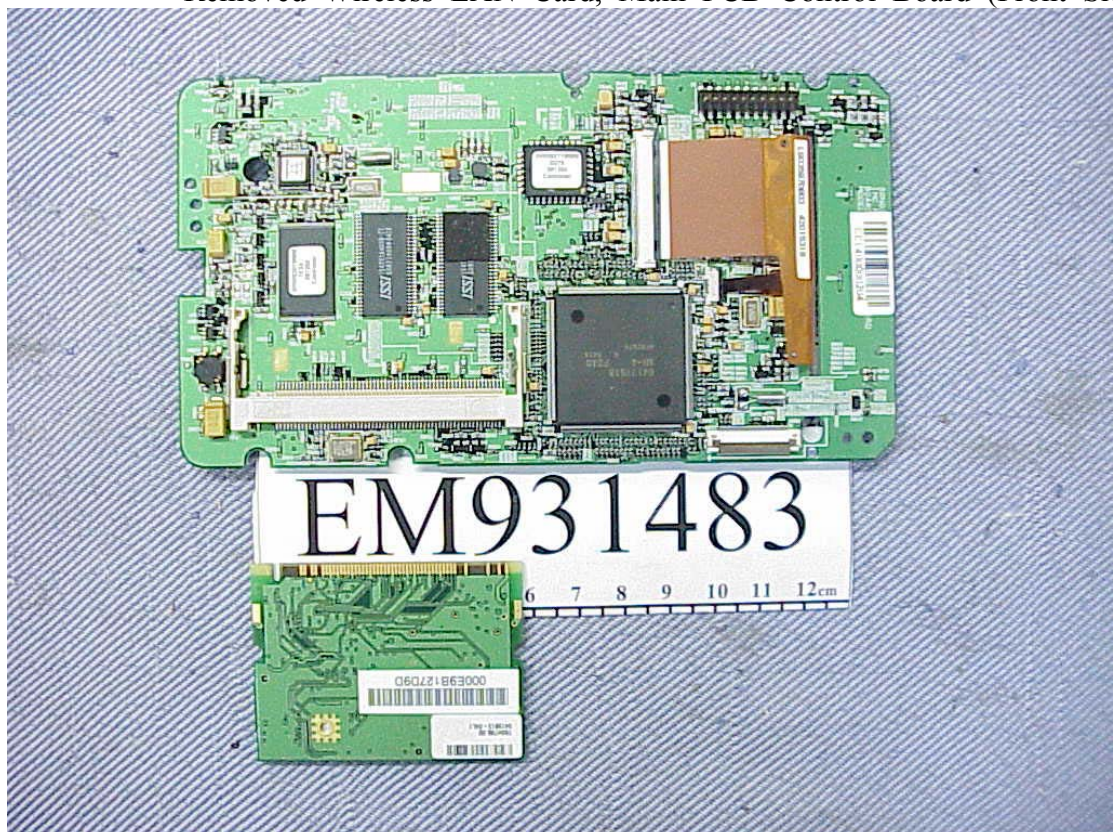
Figure 12 Removed Wireless LAN Card, Main PCB Control Board (Front Side)
