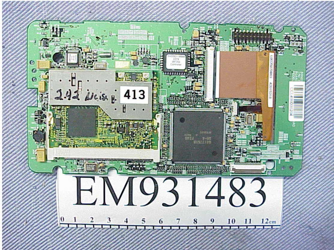
Figure 11 Main PCB Control Board w/Wireless LAN Card (Front Side)
