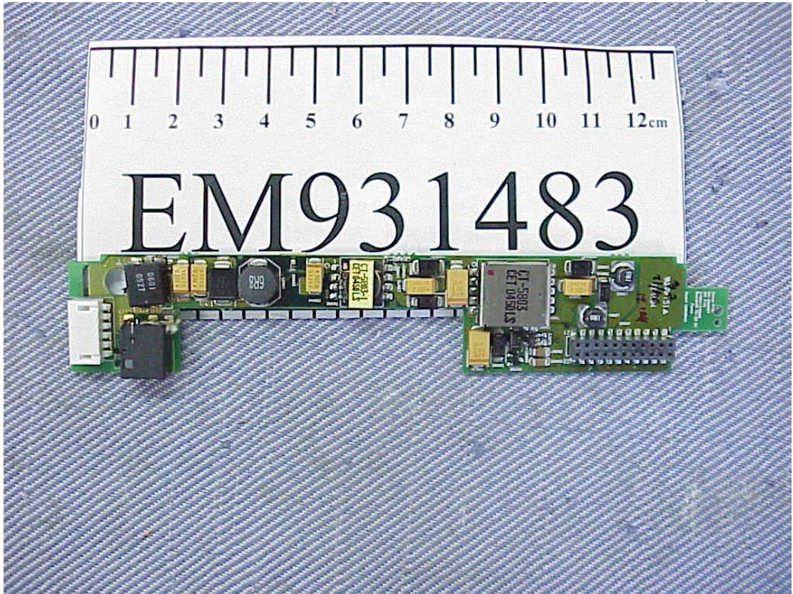
Figure 9 RX Board (Front Side)
