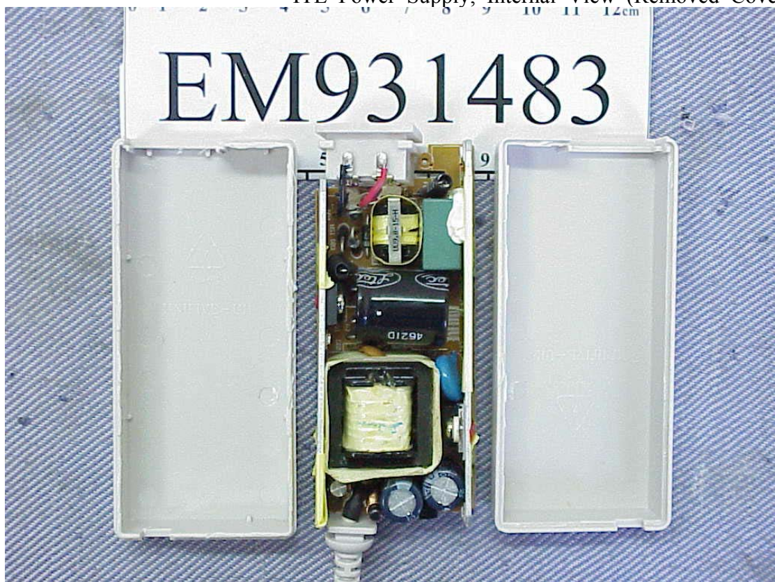
Figure 22 ITE Power Supply, Internal View (Removed Covers)
