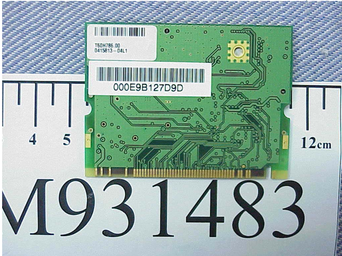
Figure 13 Wireless LAN Card (Back Side)
