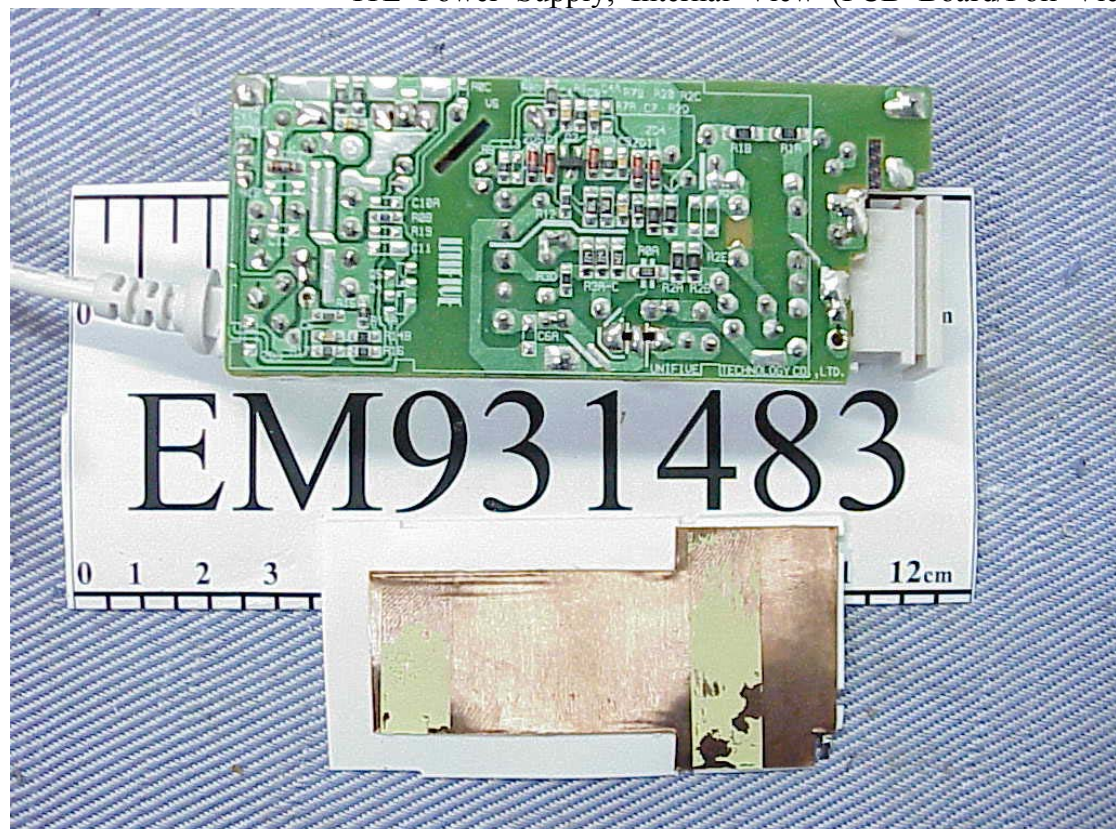
Figure 24 ITE Power Supply, Internal View (PCB Board/Foil View)
