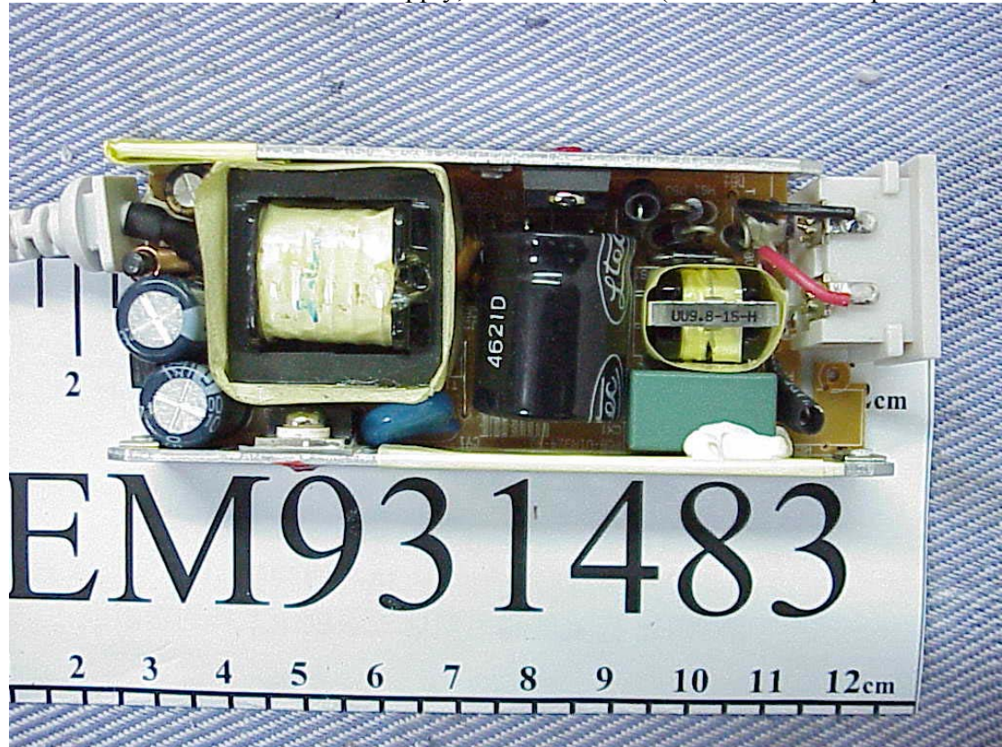
Figure 23 ITE Power Supply, Internal View (PCB Board/Component View)
