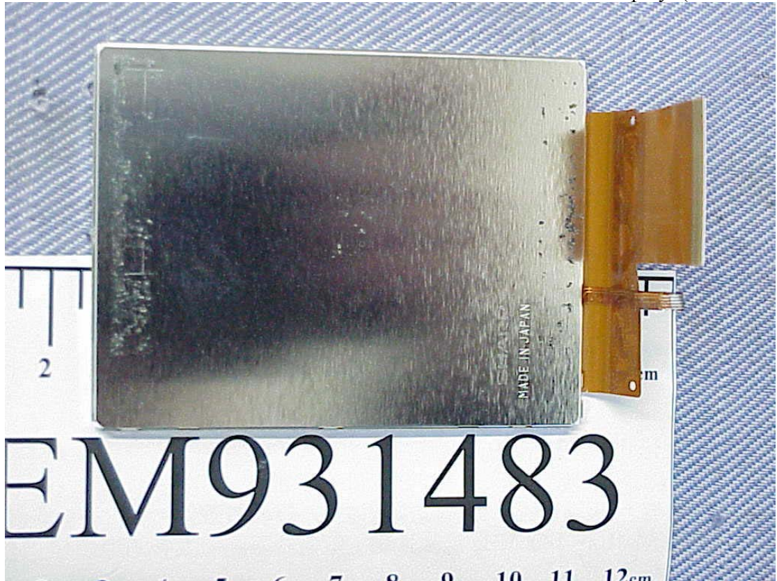
Figure 17 LCD Display (Back View)
