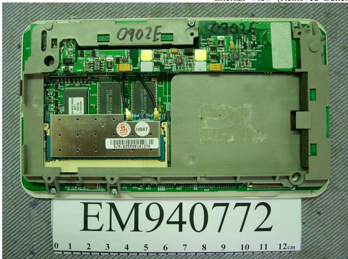
Figure 6 Internal View (Removed Battery)
