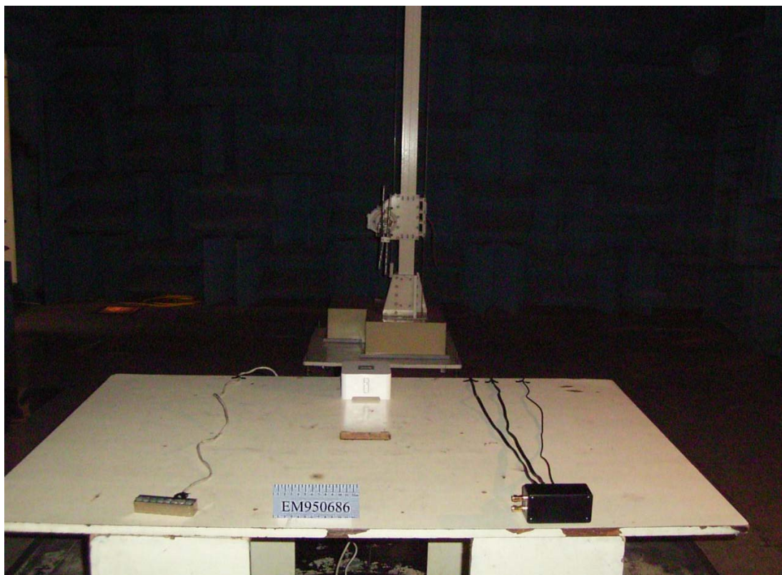
FRONT VIEW OF RADIATED MEASUREMENT
