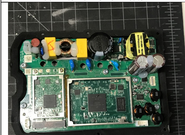
PCBA Shields Remove Top
