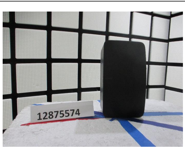
Y-ORIENTATION (LEFT)-Worst-case
