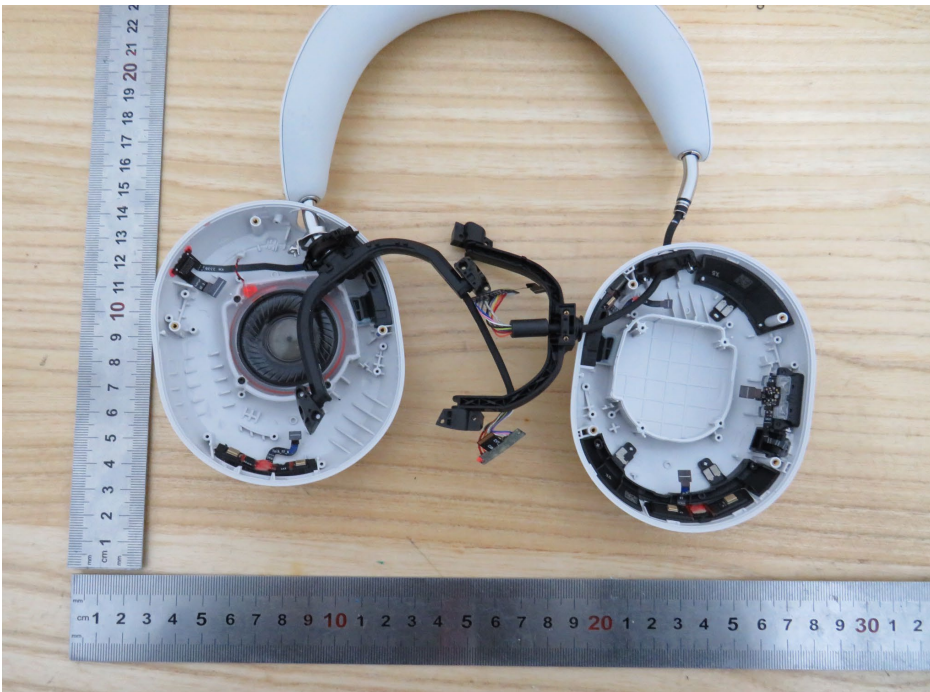
EUT Internal Photo 8
