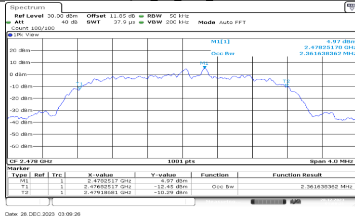
QHS_6M_Ant1_2478
