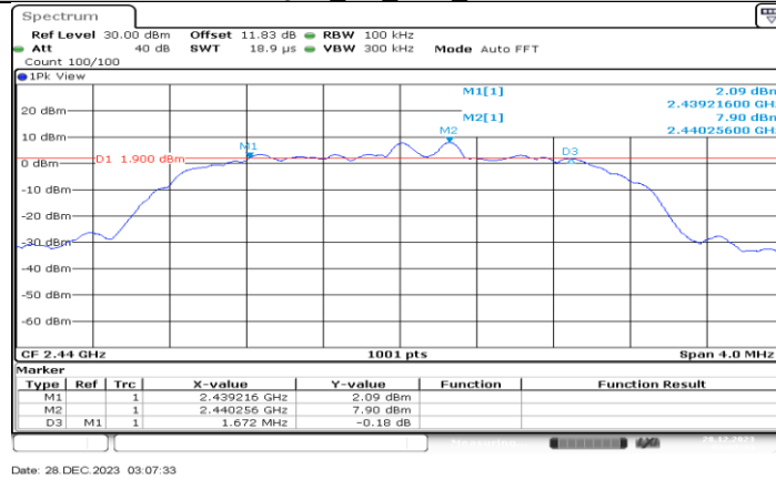
QHS_6M_Ant1_2440
