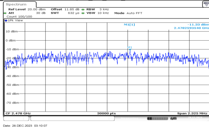
QHS_6M_Ant1_2478
