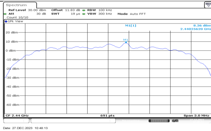
QHS_2M_Ant1_2440_0~Reference
