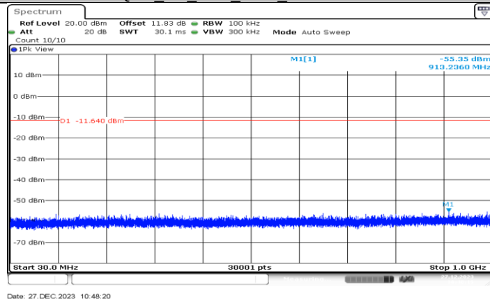
QHS_2M_Ant1_2440_30~1000
