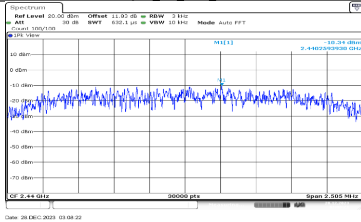
QHS_6M_Ant1_2440
