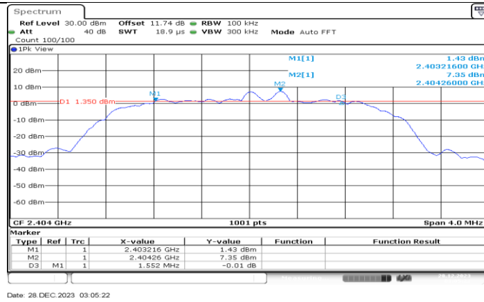
QHS_6M_Ant1_2404
