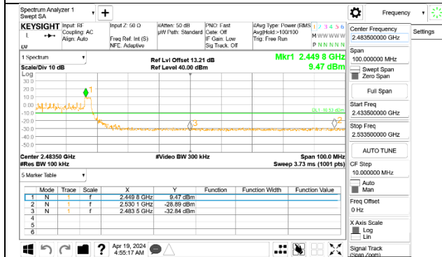
HIGH CHANNEL 7 BANDEDGE Antenna 3
