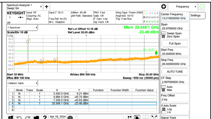
OUT-OF-BAND HIGH CHANNEL 7 Antenna 1
