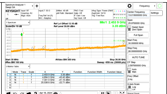
OUT-OF-BAND HIGH CHANNEL 8 Antenna 1
