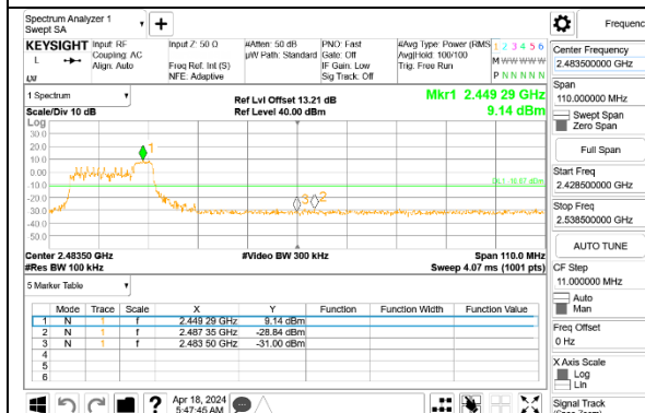
HIGH CHANNEL 7 BANDEDGE Antenna 3
