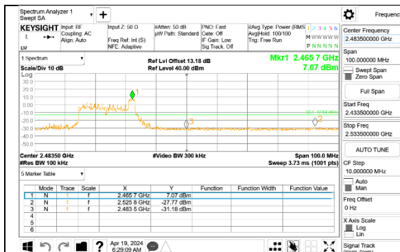
HIGH CHANNEL 10 BANDEDGE Antenna 1
