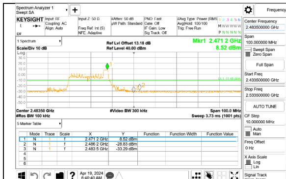
HIGH CHANNEL 11 BANDEDGE Antenna 1
