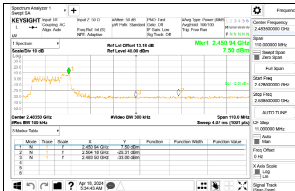
HIGH CHANNEL 7 BANDEDGE Antenna 1
