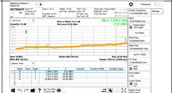
OUT-OF-BAND HIGH CHANNEL 10 Antenna 3
