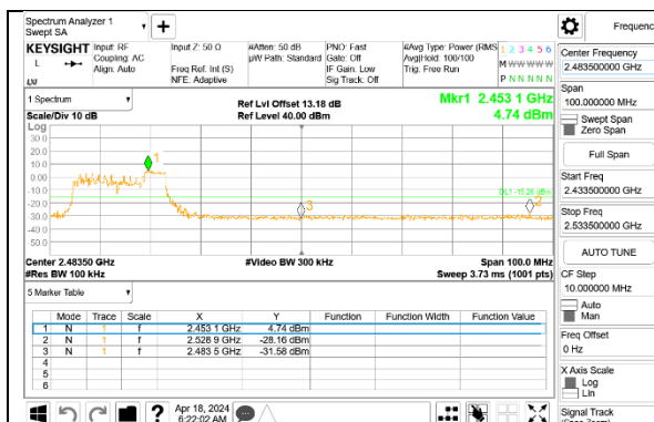
HIGH CHANNEL 8 BANDEDGE Antenna 1
