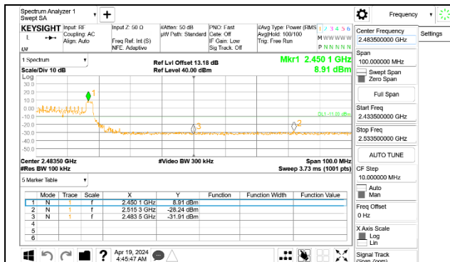
HIGH CHANNEL 7 BANDEDGE Antenna 1
