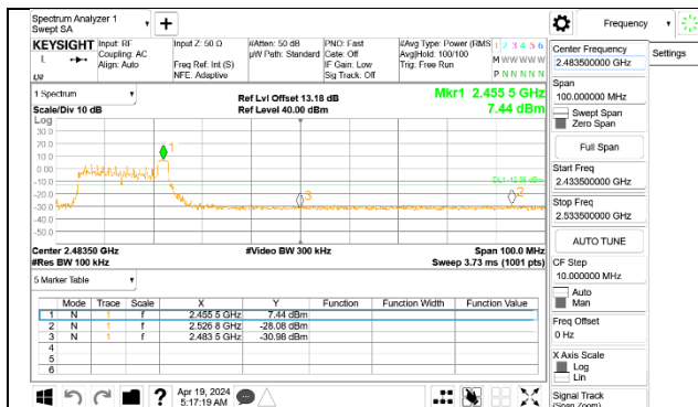
HIGH CHANNEL 8 BANDEDGE Antenna 1
