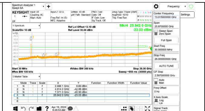
OUT-OF-BAND HIGH CHANNEL 10 Antenna 1
