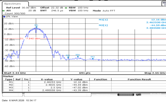
11B-CDD_Ant2_High_2462
