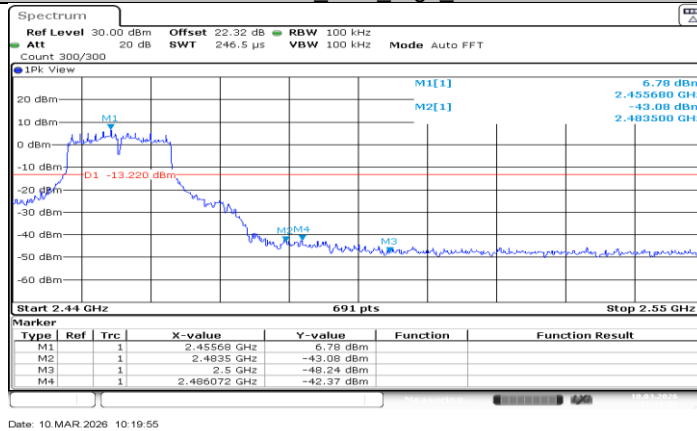
11G-CDD_Ant2_High_2457
