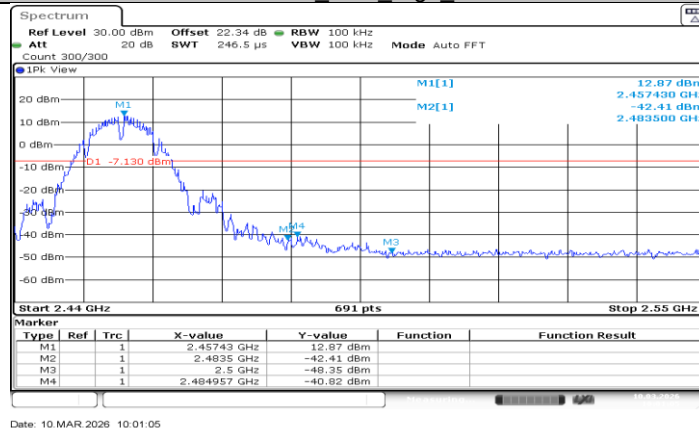
11B-CDD Ant1_High_2457
