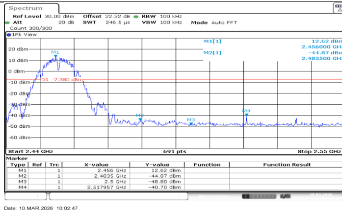
11B-CDD_Ant2_High_2457
