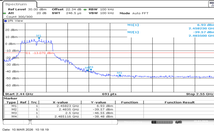
11G-CDD_Ant1_High_2457
