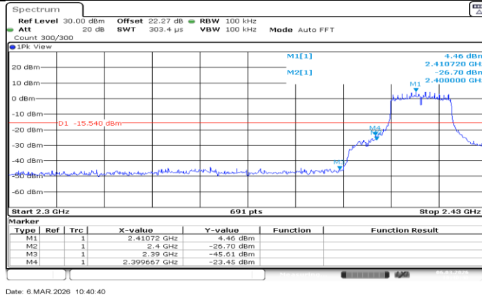
11G-CDD_Ant2_Low_2412
