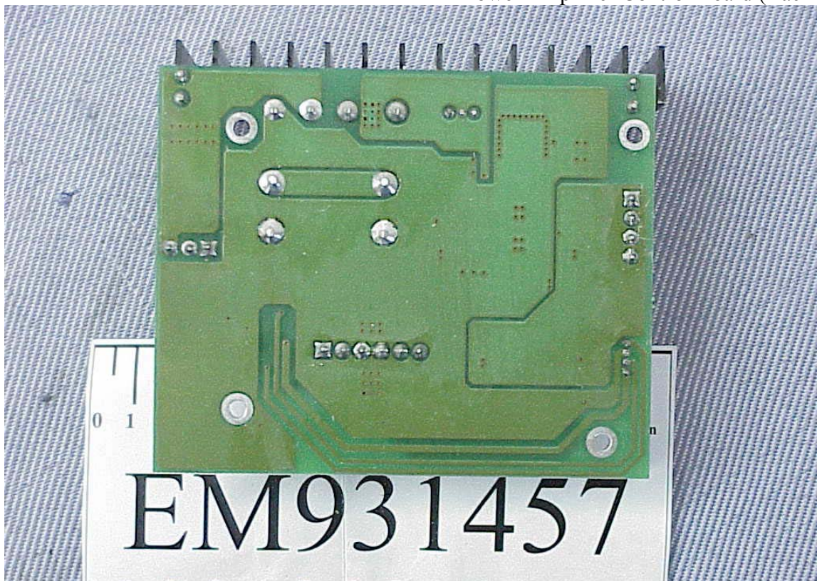
Figure 24 Power Amplifier Control Board (Back Side)
