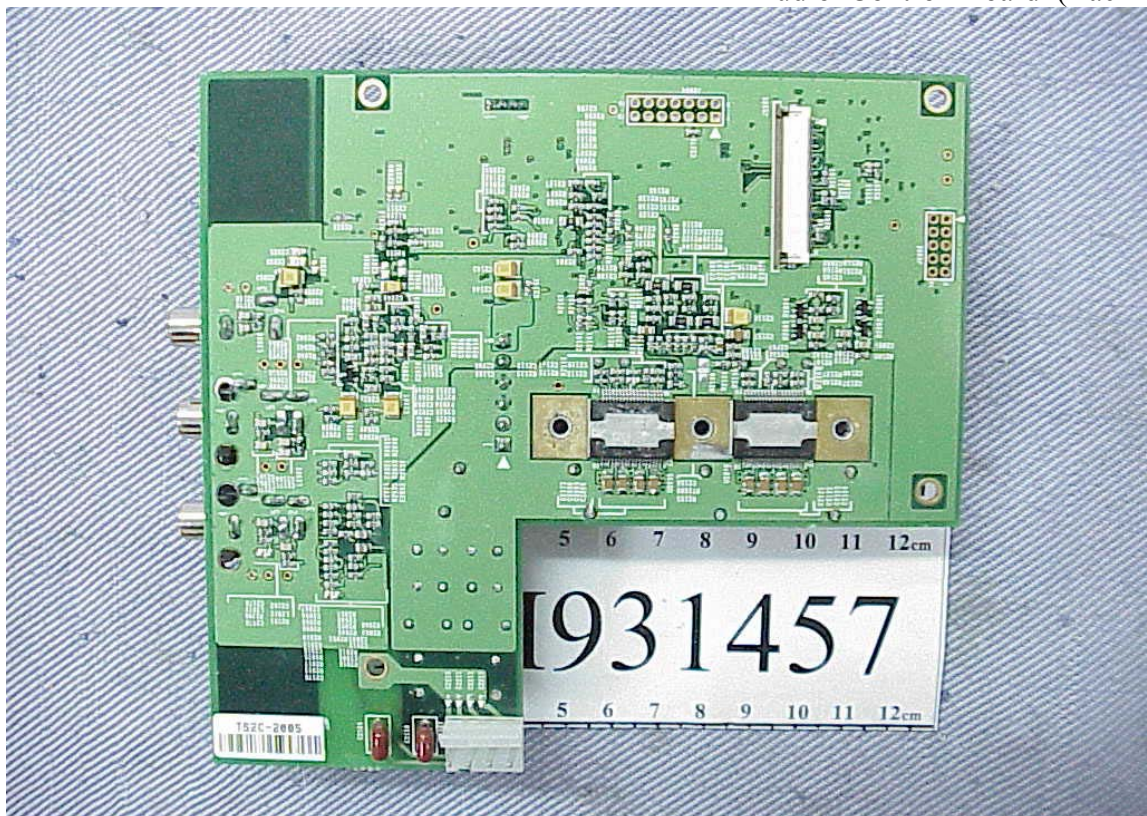
Figure 18 Audio Control Board (Back Side)
