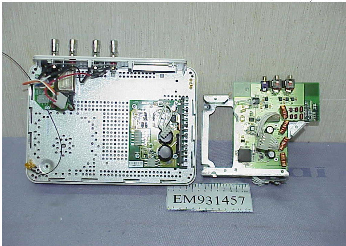
Figure 16 Removed Audio Control Board, Internal View
