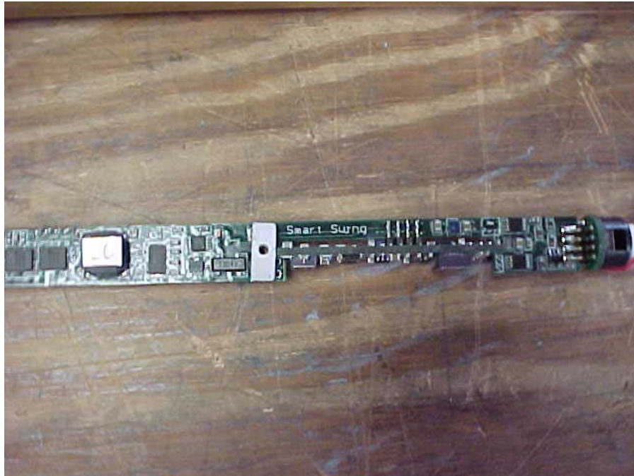
Internal Circuit Board – End View
