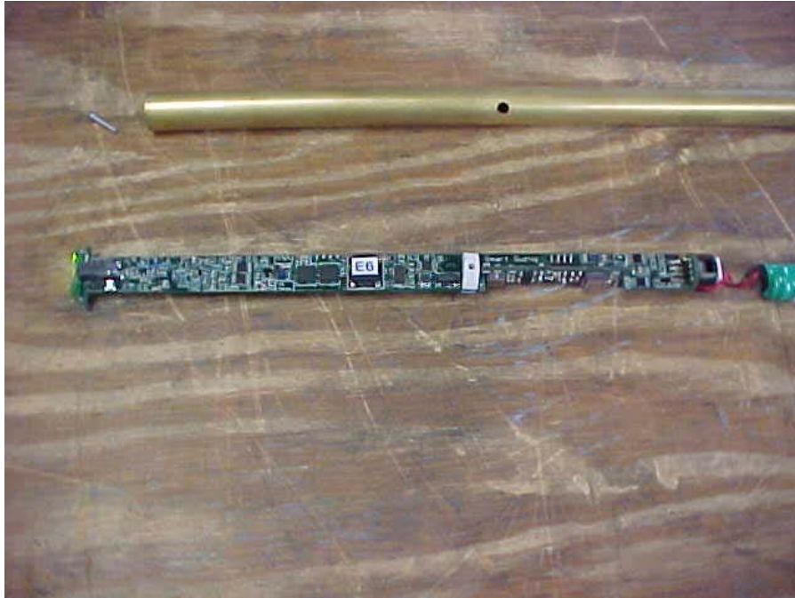
Internal Circuit Board in Smart Swing Golf Club Handle
