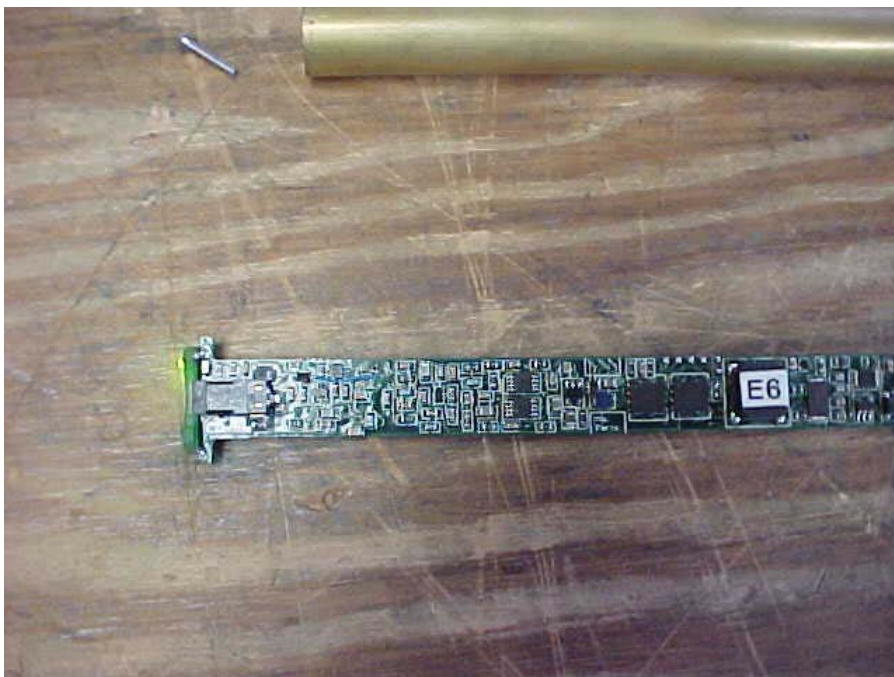
Internal Circuit Board – Top View
