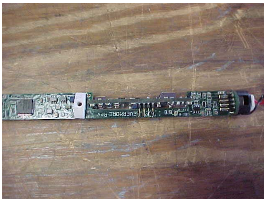
Internal Circuit Board – Bottom Closeup
