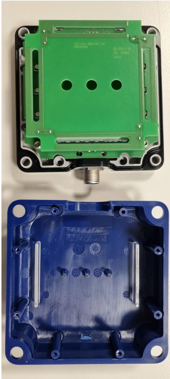
Picture 1. A cover disassembled from B cover. RFID antenna is mounted at the top of main pwb.
