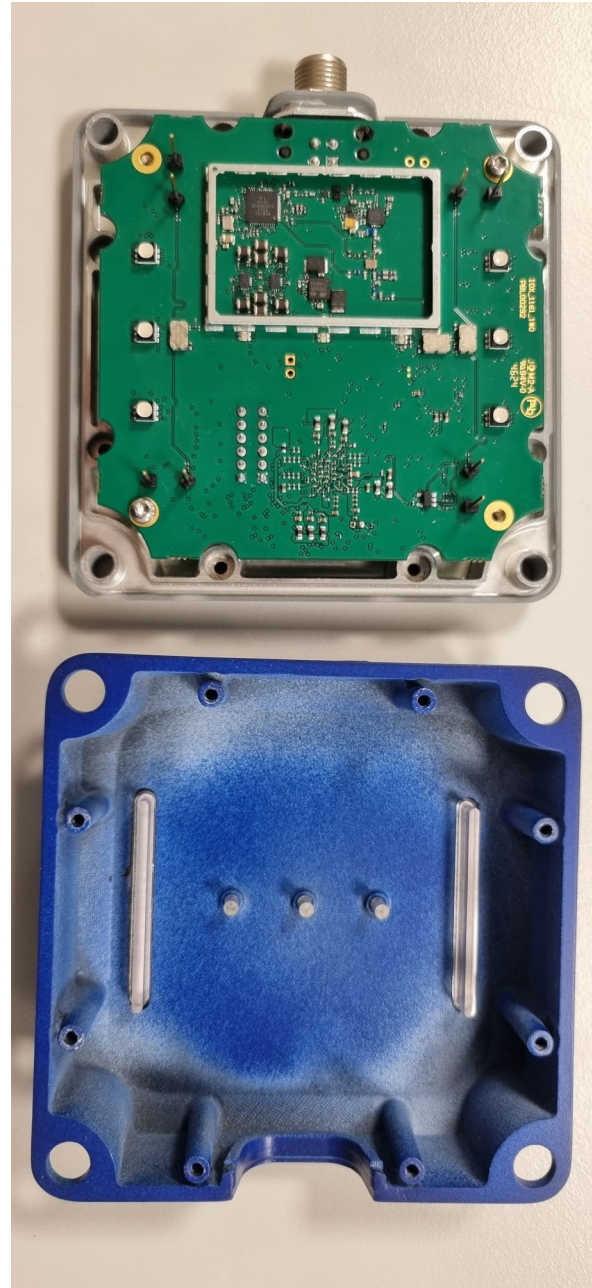
Pic 2. Antenna removed from main pwb. RF shield removed from RFID radio parts.
