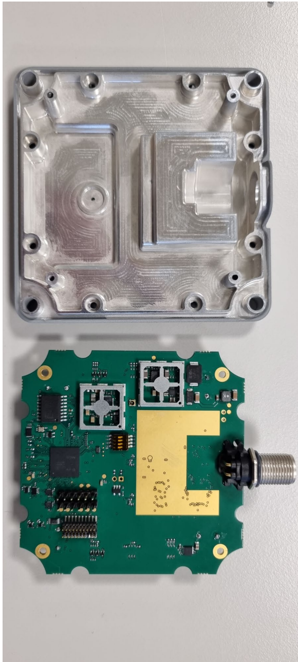
Pic 3. IOX100 main pwb bottom side and B Cover. Pic 4. IOX100 main pwb and antenna. RFID radio parts without shield.
