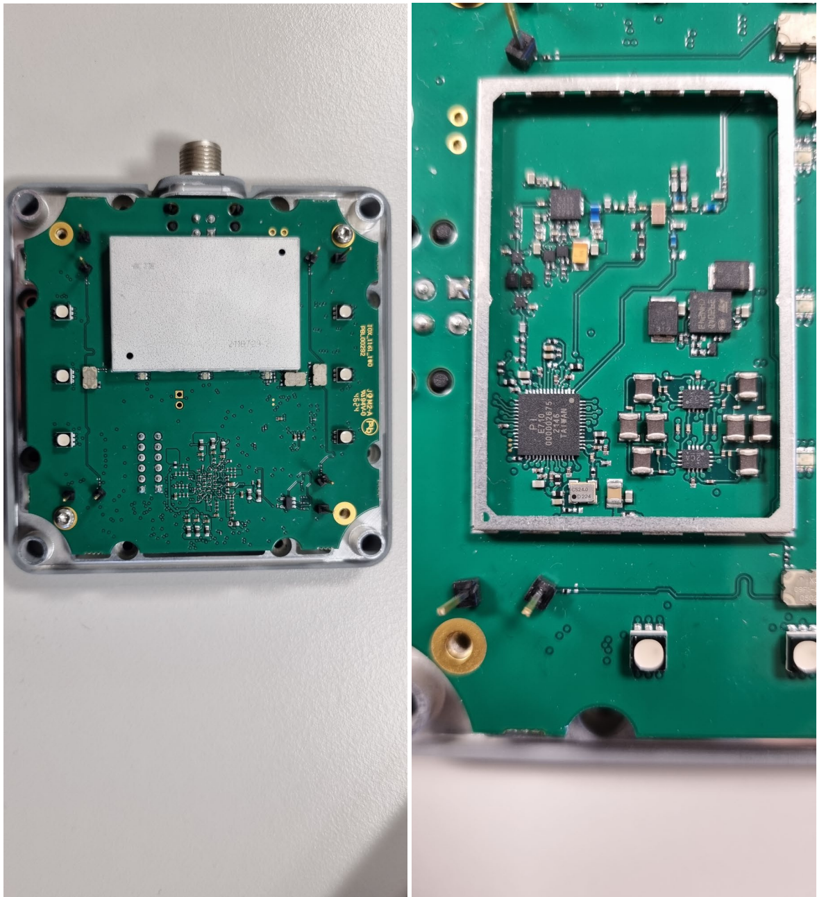
Picture 5 & 6. IOX100 RFID radio parts with RF shield and closer look without shield.
