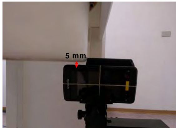
Fig.6 EUT right side (slant) to flat phantom
