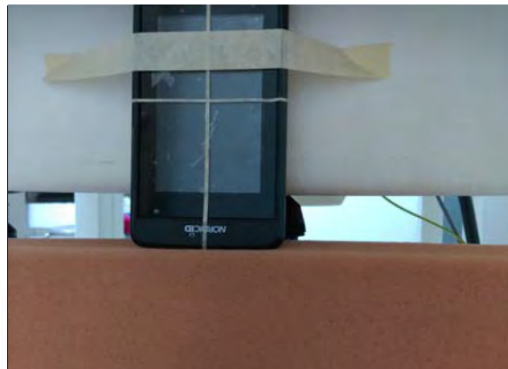
Fig.11 EUT Inner surface_2 to flat phantom
