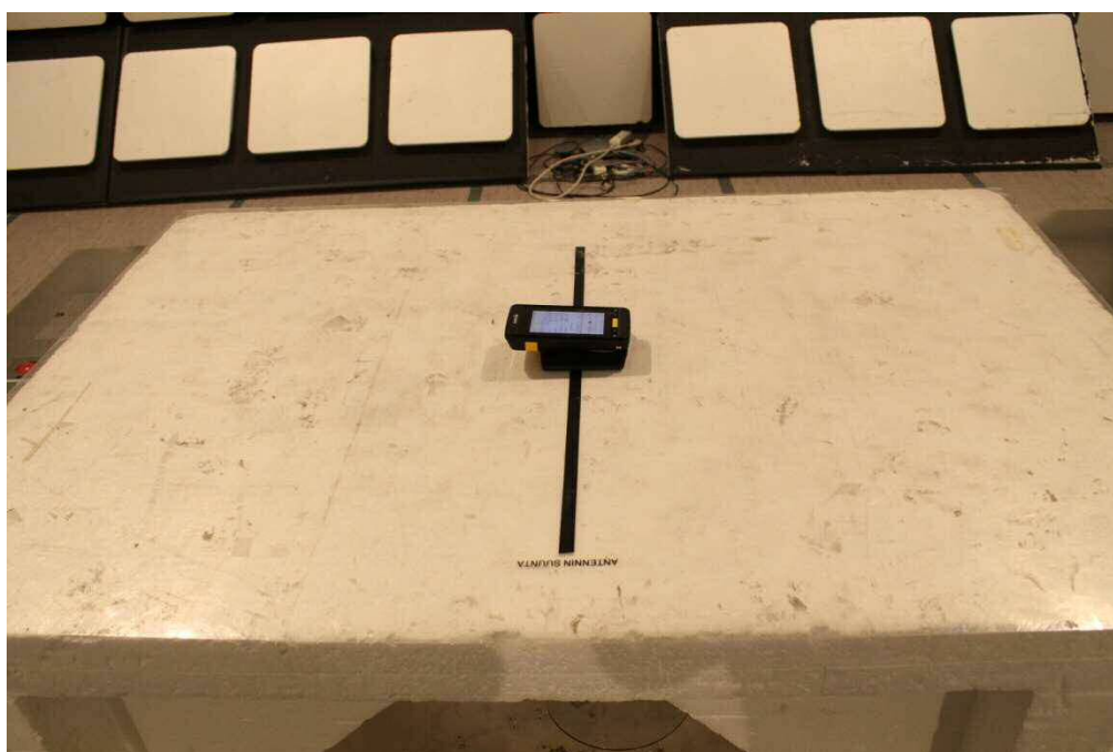
Photograph 4. EUT on table
