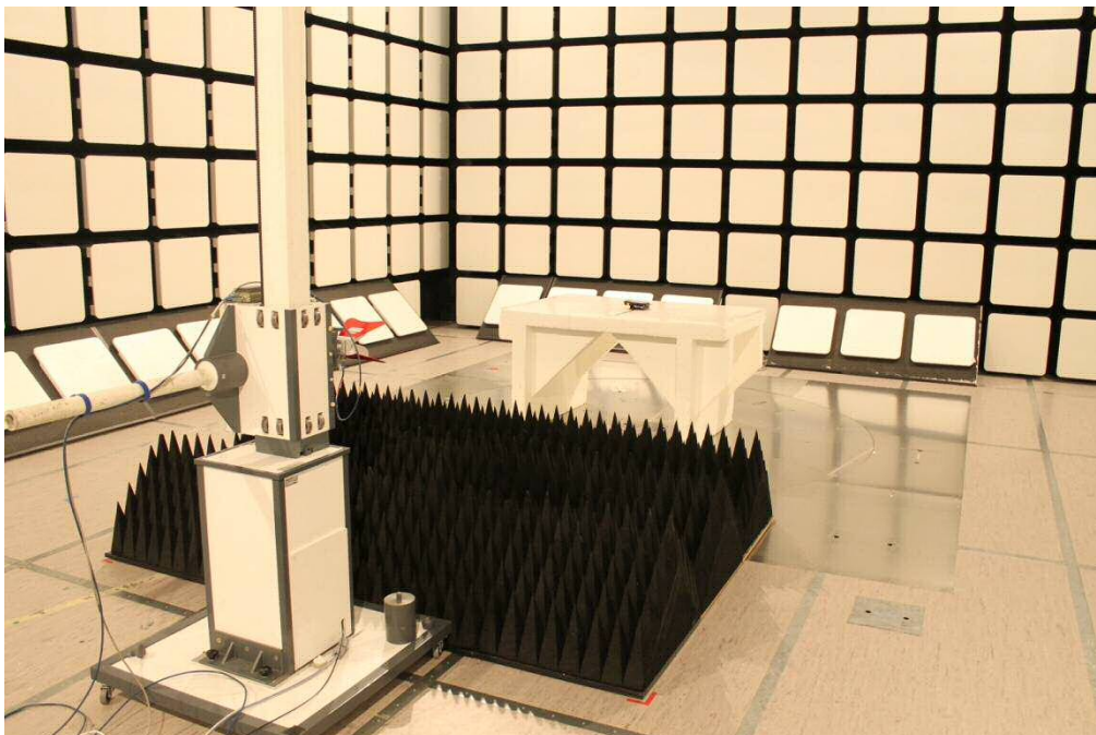
Photograph 2. Radiated Spurious Emissions 1 – 18 GHz
