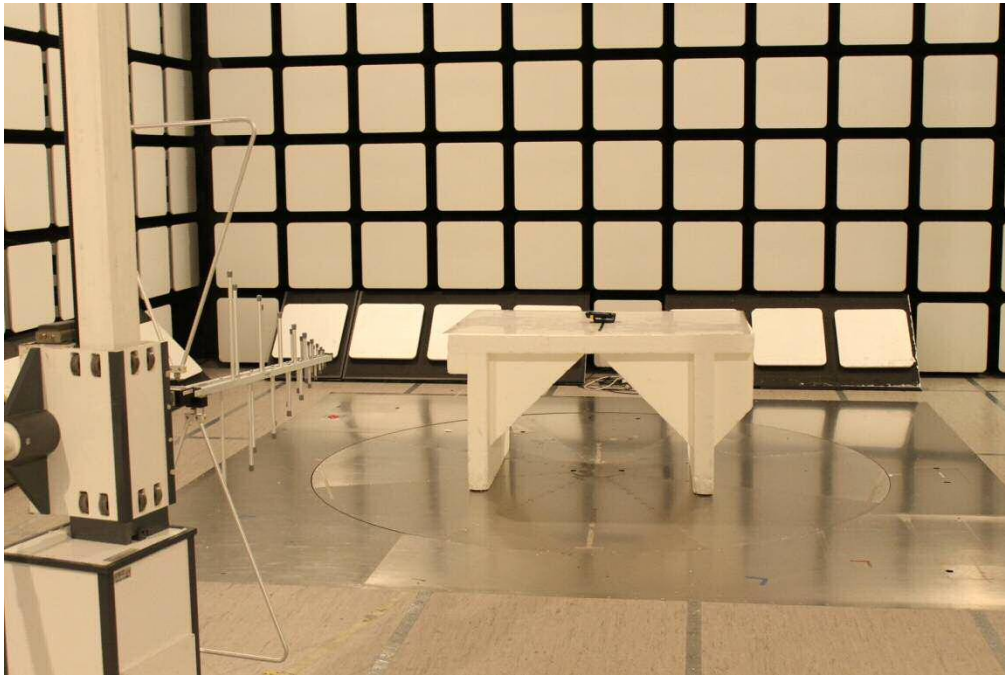
Photograph 1. Radiated Spurious Emissions 30 – 1000 MHz
