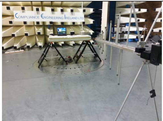
Fig 5 Radiated Emissions
