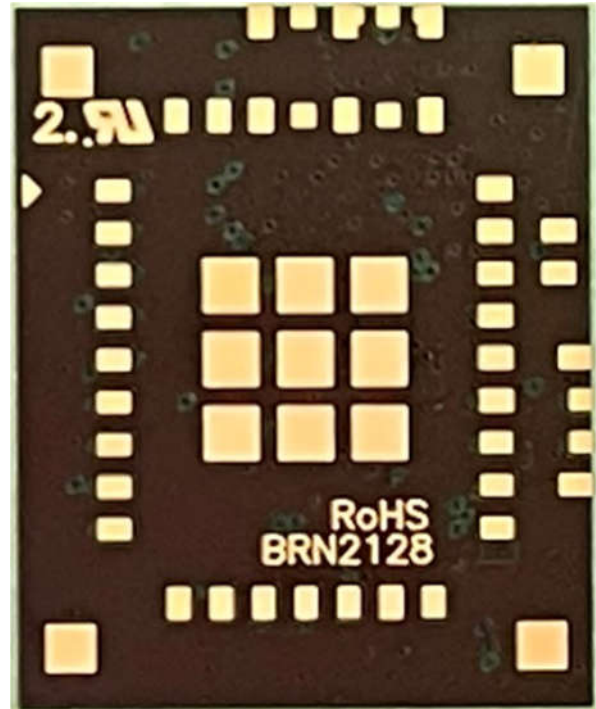
Picture 2. NUR3-1W module bottom side
