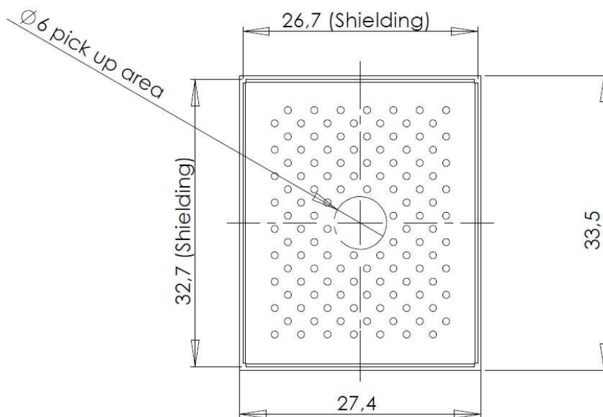
Picture 9. Mechanical dimension top view of the NUR3-1W.
