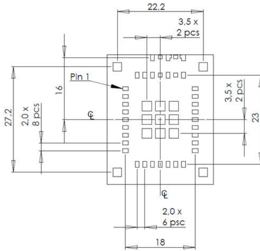
Picture 11. Mechanical dimension bottom view of the NUR3-1W.
