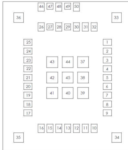
Picture 2. NUR3-1W pad numbering (top thru view).
