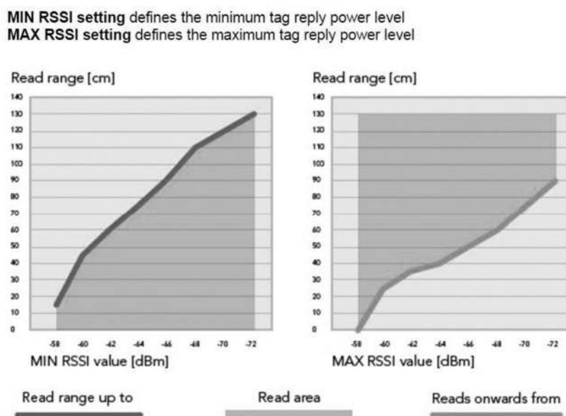
Picture 7. Read range limited by RSSI filters (100mW TX power level with 0dBi antenna gain used).
