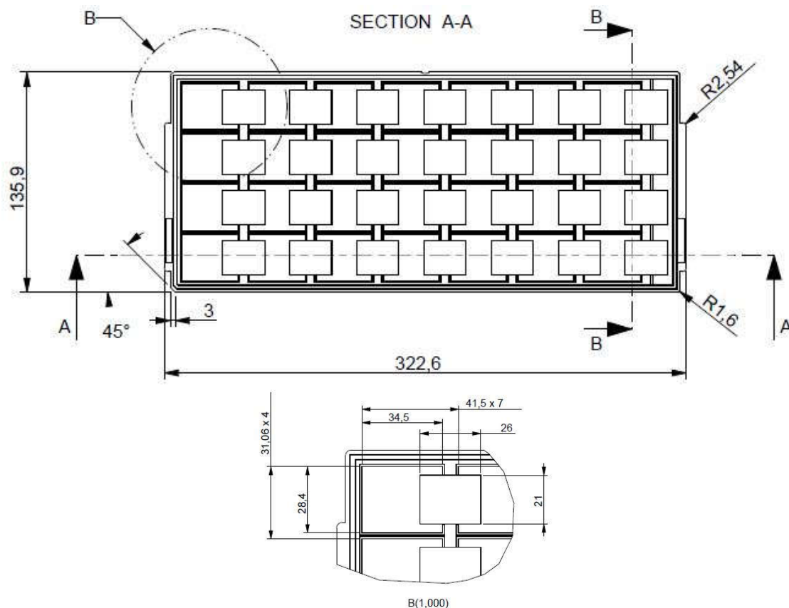
Picture 13. NUR3-1W packing tray dimensions.
