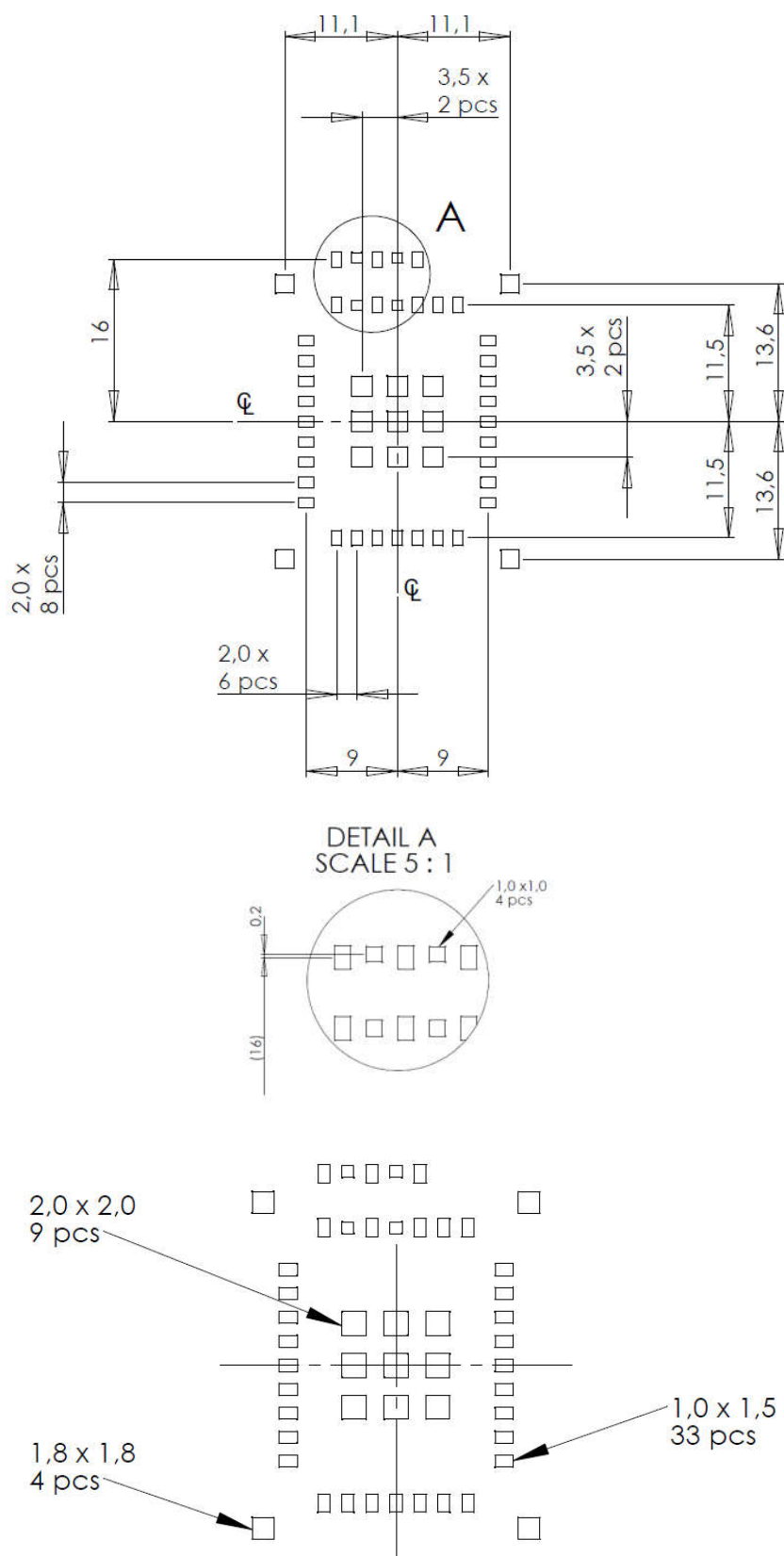
Picture 12. Land pattern of the NUR3-1W module.
