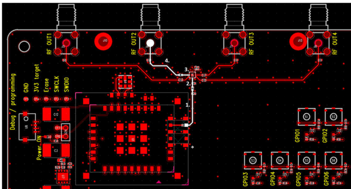
Picture 5. NUR3-1W module EVB RF path used in certifications.
