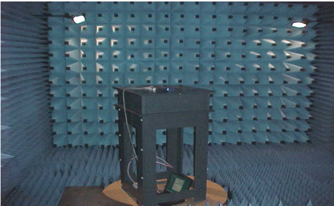
Spurious emission 1-26 GHz
