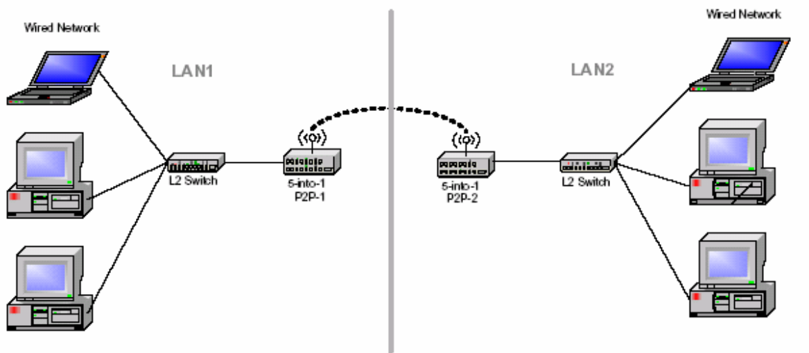
Figure 5: P2P Mode (Wireless Bridge)
