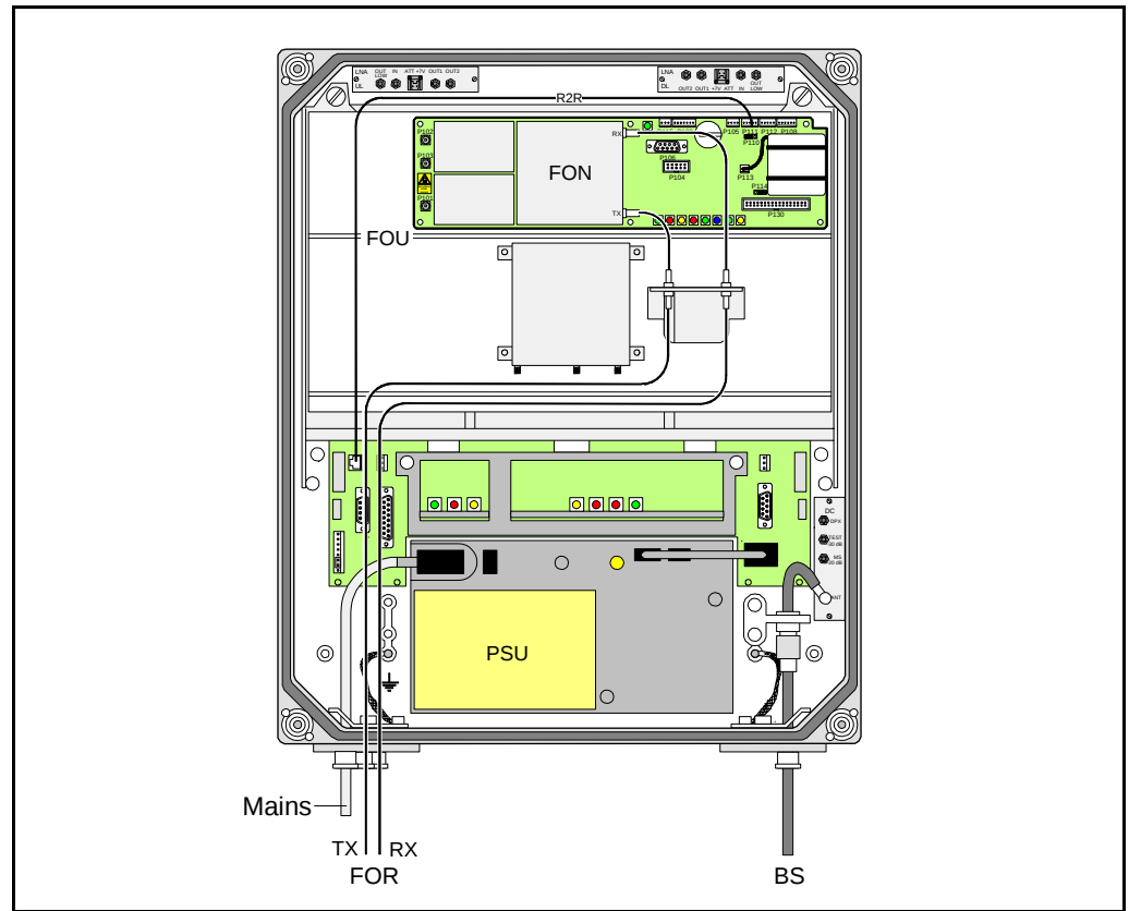
Figure 3-10. Connecting RMU
