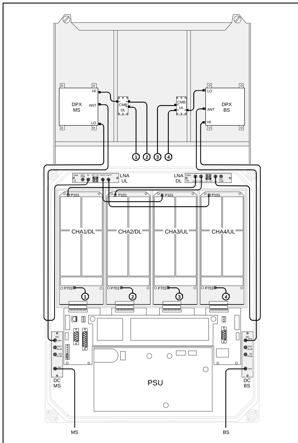
Figure 5-25. Cabling, 4 channel GSM repeater
