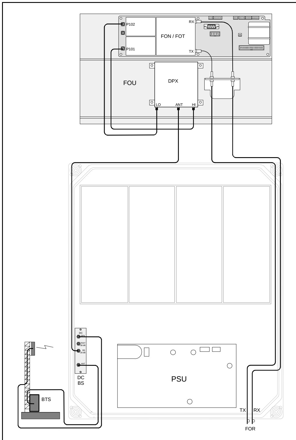
Figure 5-30. Cabling, BMU
