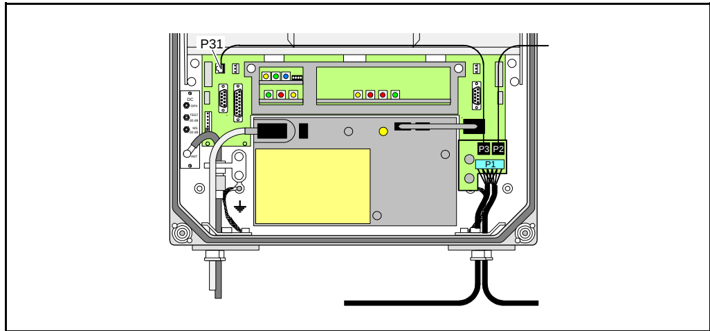
Figure 3-13. R2R connection
