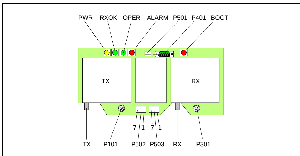
Figure 5-22. FOT indicators and ports
