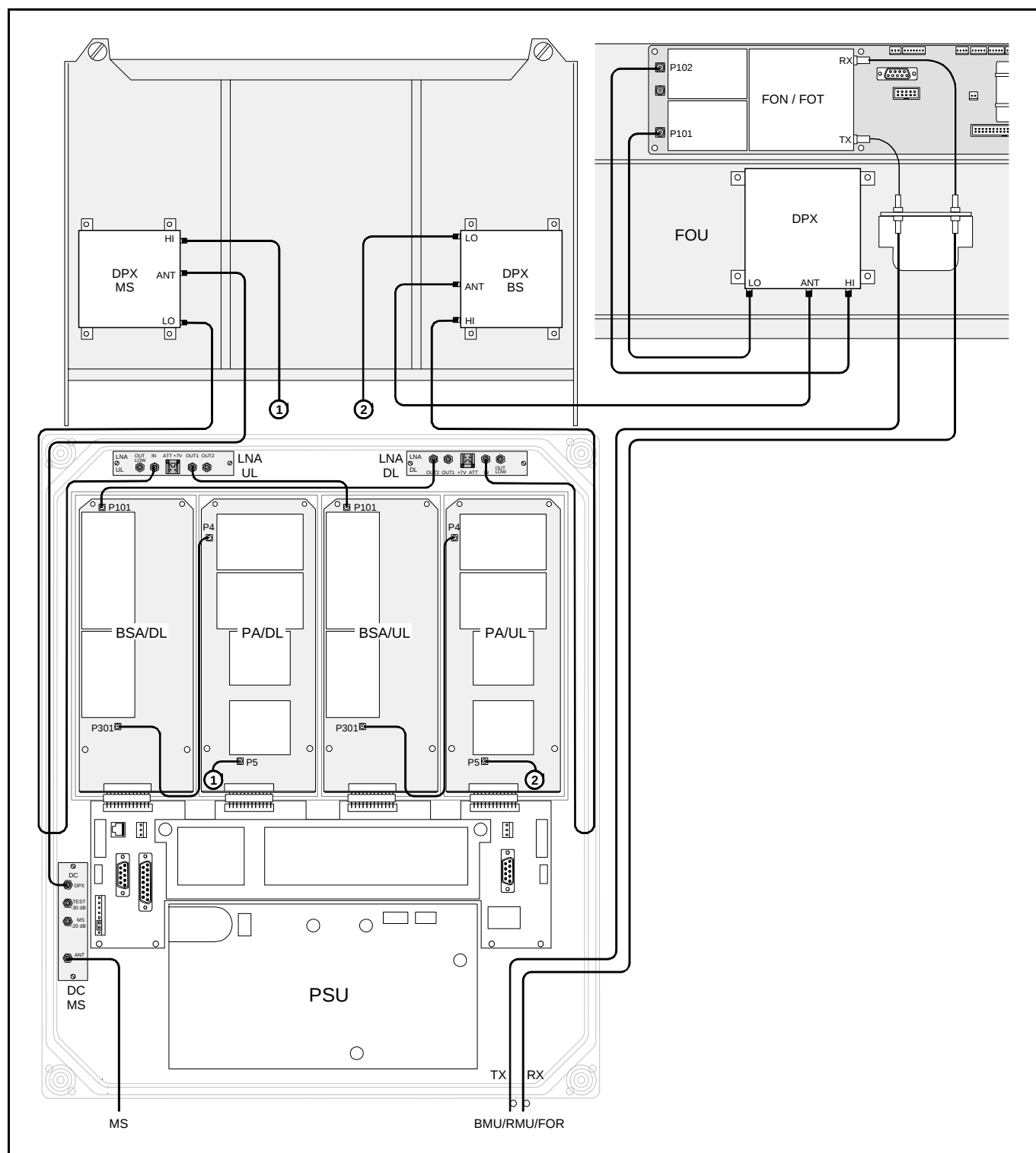
Figure 5-32. Cabling, FOR
