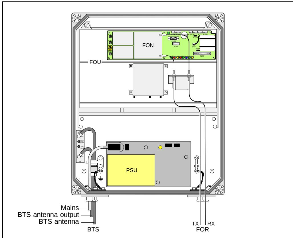
Figure 3-9. Connecting BMU
