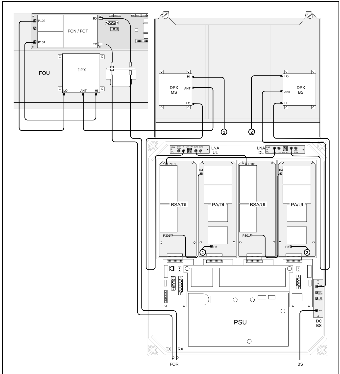
Figure 5-31. Cabling, RMU
