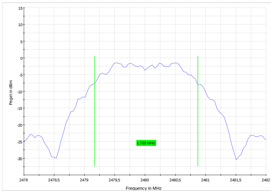
6 dB Bandwidth
