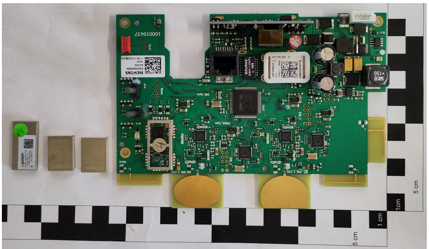
PCB uncovered
