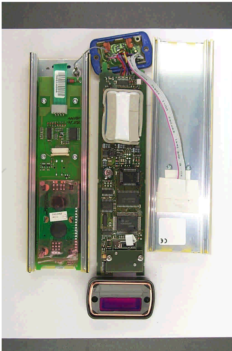
40694eut14.jpg: EUT, internal view
