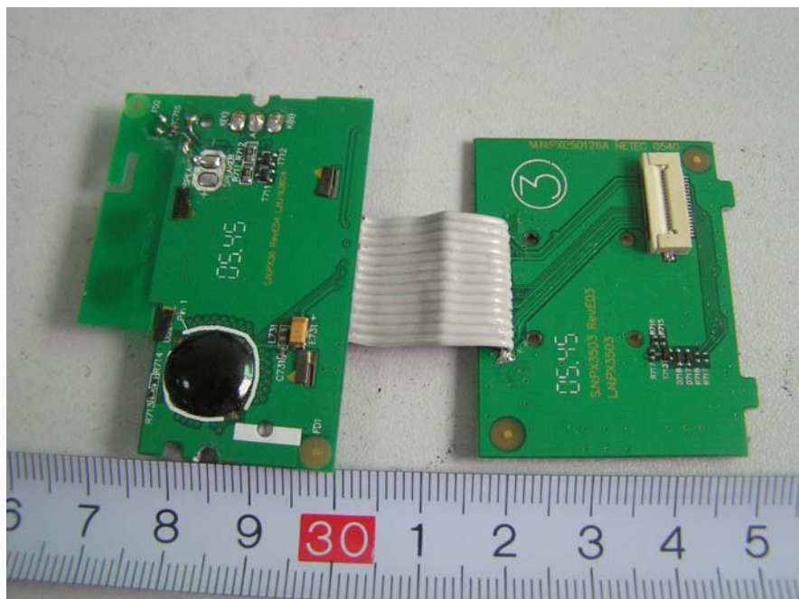
EUT –LCD & Keyboard Rear View
