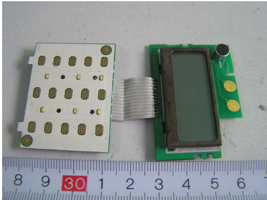
EUT –LCD & Keyboard Front View
