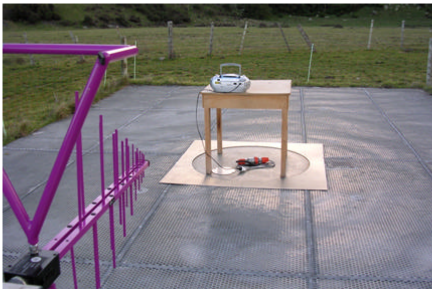
Figure 5: Measurement Test Set-up
