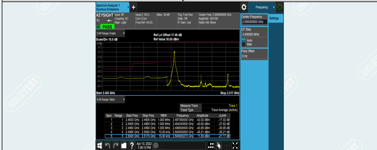
Band7-15MHz-16QAM-20825-1RB#0
