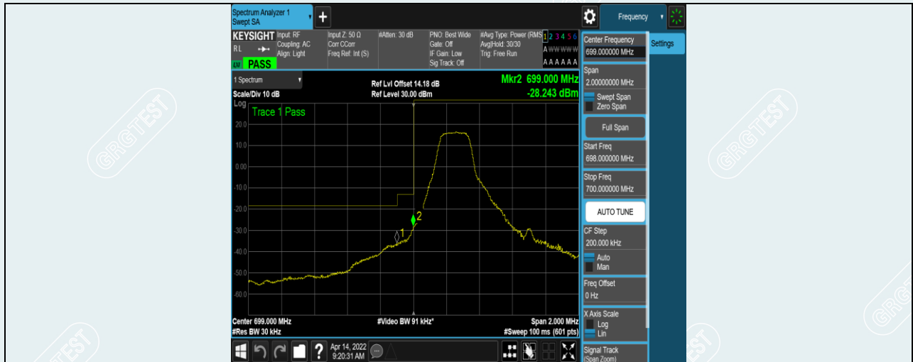
Band12-1.4MHz-QPSK-23017-1RB#0
