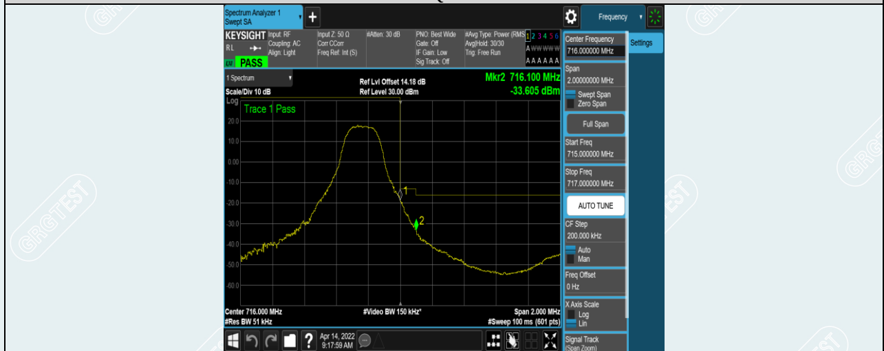
Band12-3MHz-16QAM-23165-1RB#14
