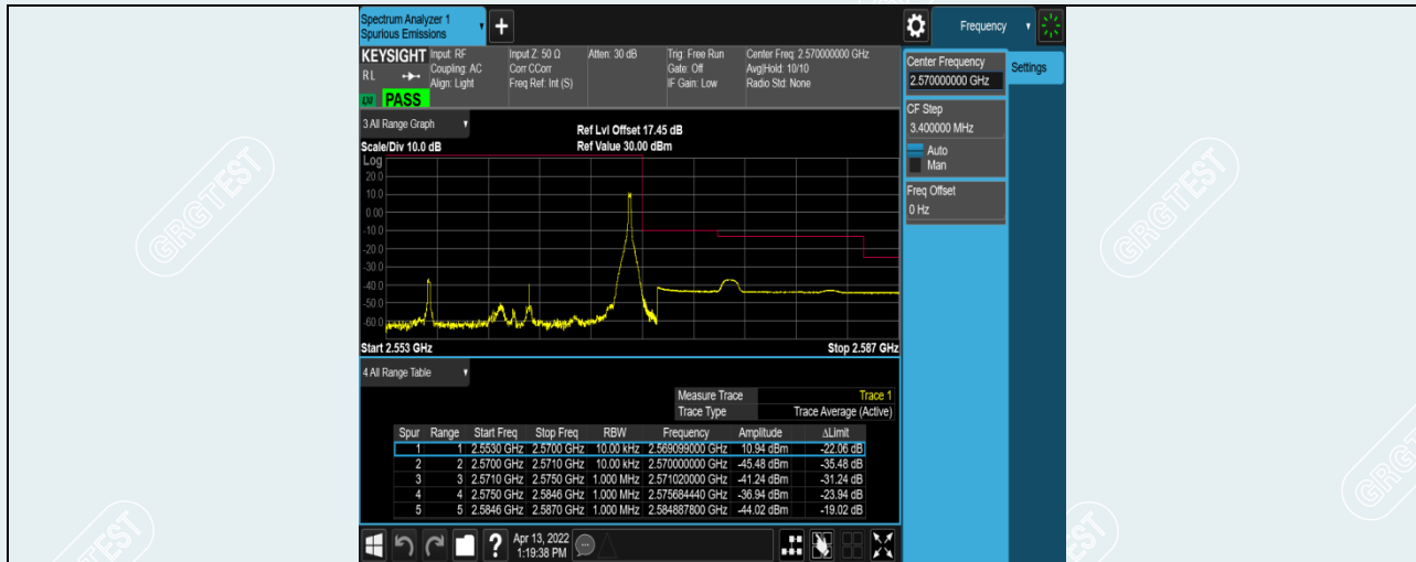
Band7-15MHz-QPSK-21375-1RB#74
