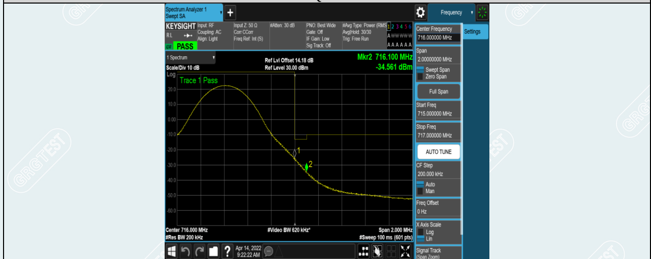
Band12-10MHz-QPSK-23130-1RB#49
