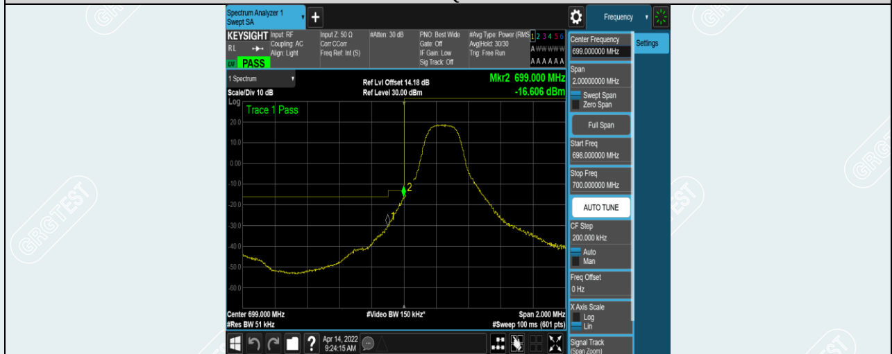
Band12-3MHz-QPSK-23025-1RB#0
