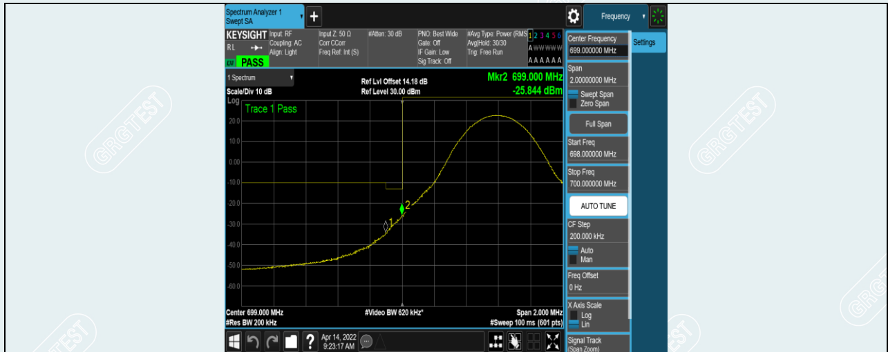
Band12-10MHz-QPSK-23060-1RB#0
