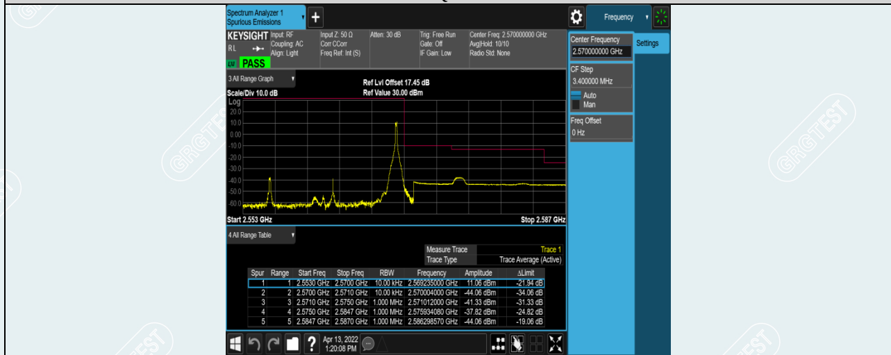
Band7-15MHz-16QAM-21375-1RB#74
