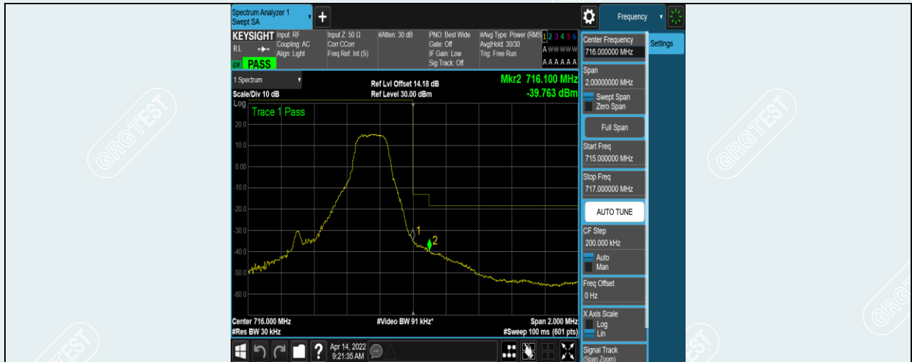
Band12-1.4MHz-16QAM-23173-1RB#5
