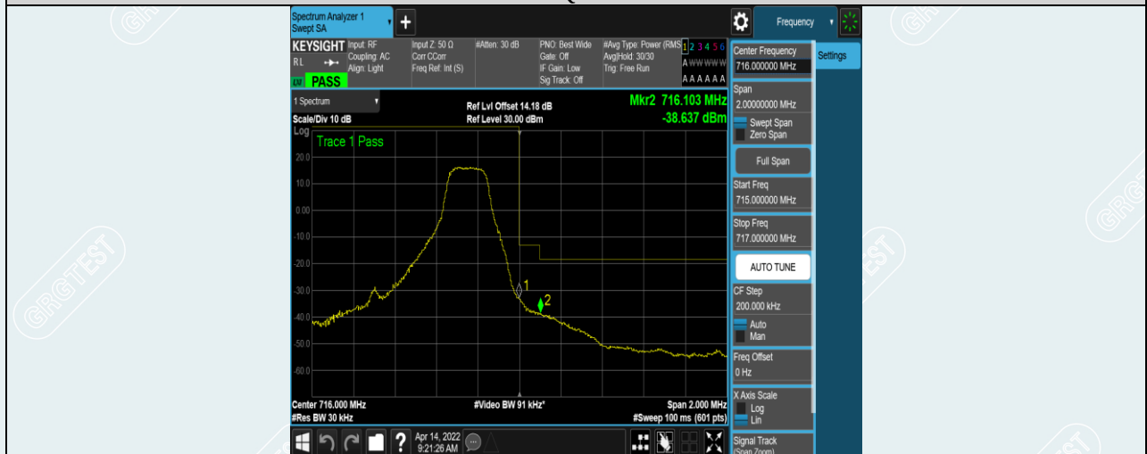
Band12-1.4MHz-QPSK-23173-1RB#5
