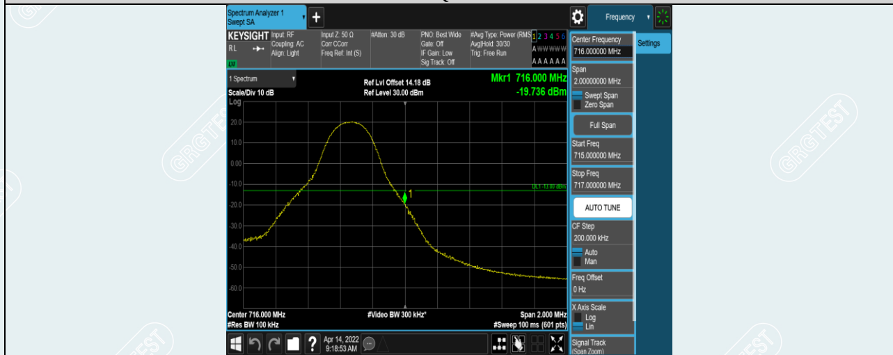
Band12-5MHz-16QAM-23155-1RB#24
