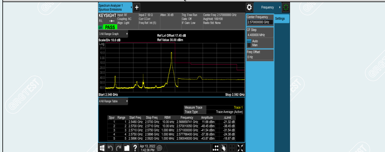
Band7-20MHz-QPSK-21350-1RB#99
