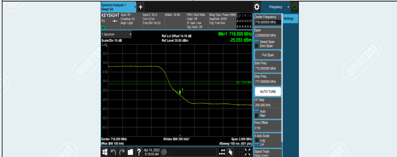
Band12-5MHz-QPSK-23155-25RB#0
