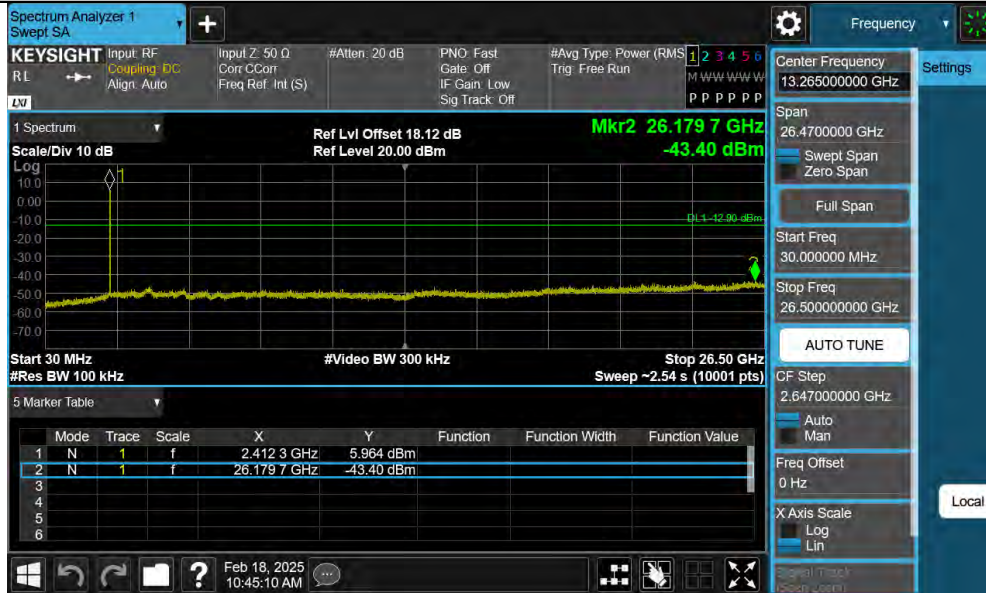
11B-Ant2-2412-30~26500-PASS
