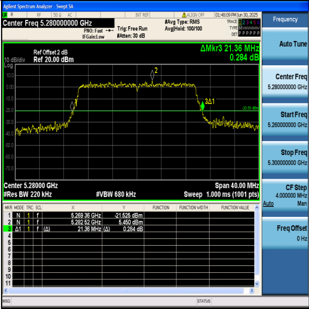
11AX20SISO-Ant1-5280
