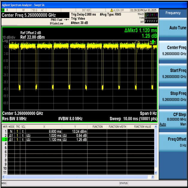
NTNV-11AX20SISO-Ant1-5260
