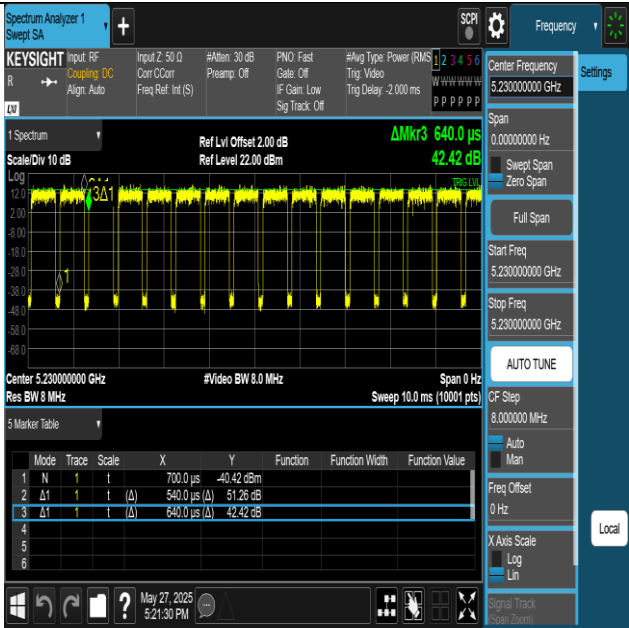
NTNV-11AX40SISO-Ant1-5230
