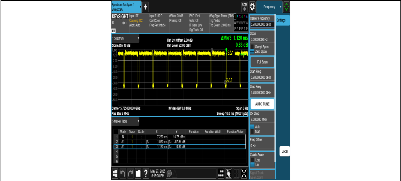
NTNV-11AX20SISO-Ant1-5785
