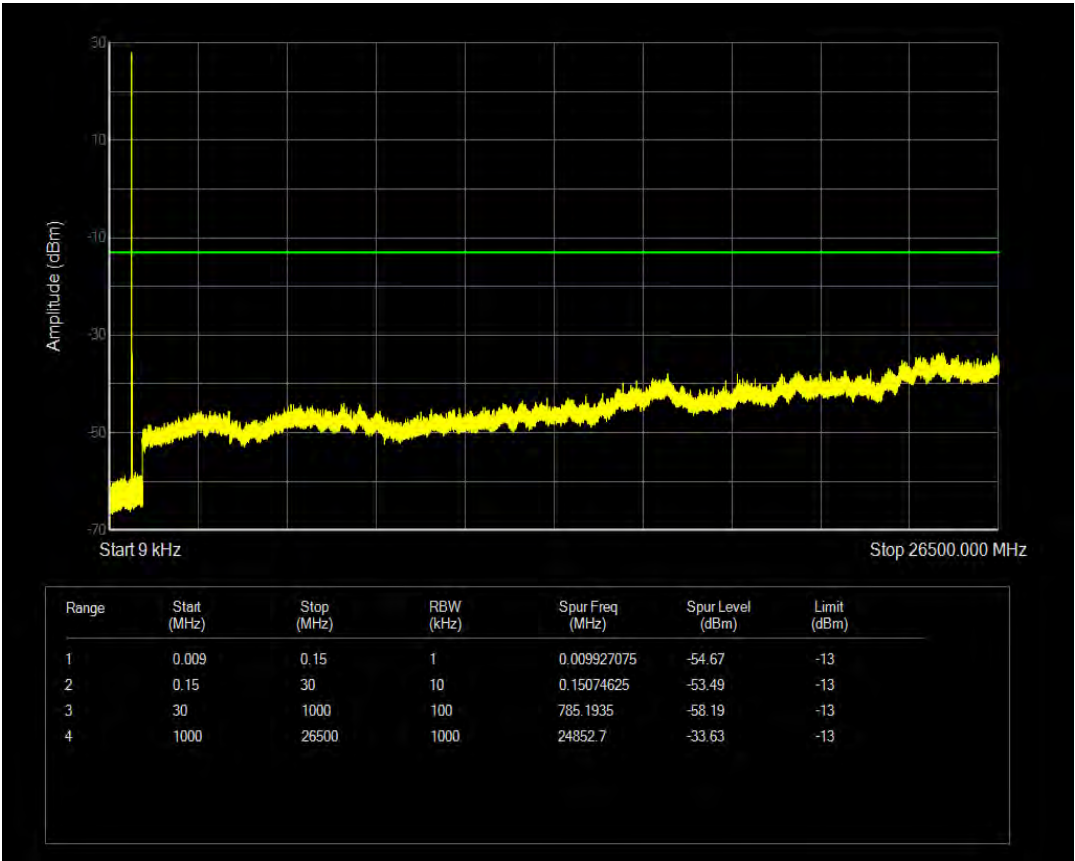
n71 SCS=15kHz CP QPSK BW=15MHz Channel=136100 RB=1@78
