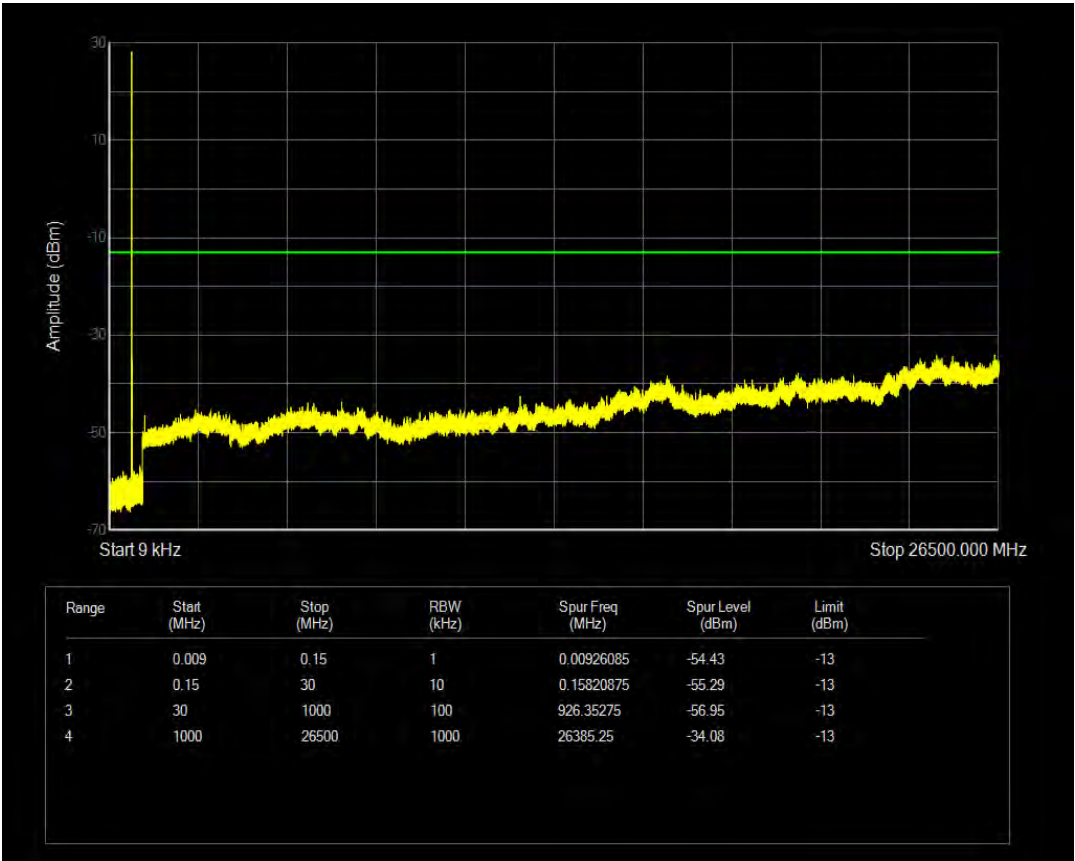
n71 SCS=15kHz CP QPSK BW=5MHz Channel=136100 RB=1@24
