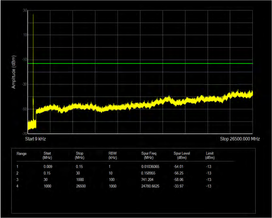
n71 SCS=15kHz CP QPSK BW=5MHz Channel=136100 RB=1@0
