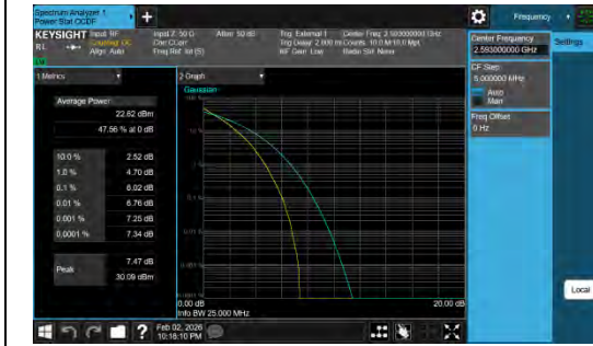
Band41-20MHz-QPSK-40620-100RB#0-PASS
