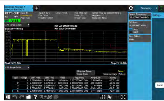
Band41-20MHz-QPSK-41490-100RB#0-PASS
