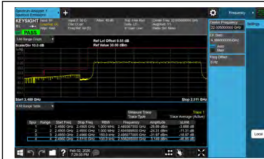
Band41-20MHz-QPSK-39750-100RB#0-PASS
