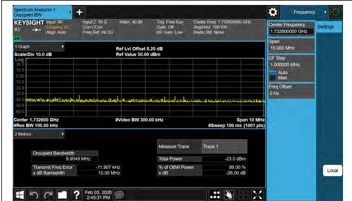
Band4-1413-3-PASS
