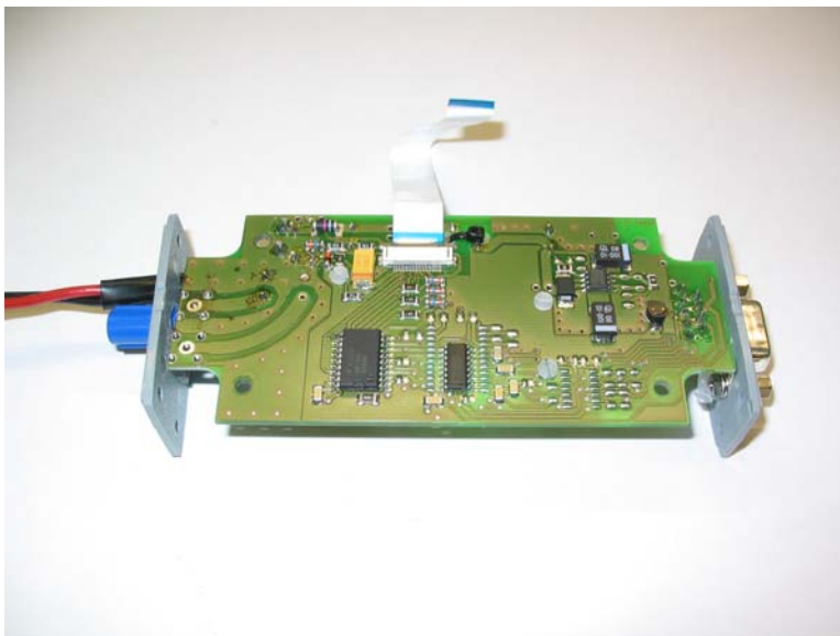
Bottom of PCB 1
