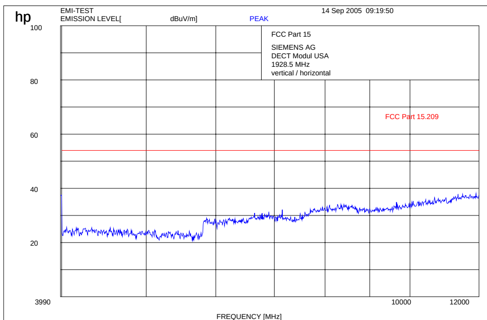
Plot 8: 4 GHz – 12 GHz Transmitter radiated (1928.5 MHz)
