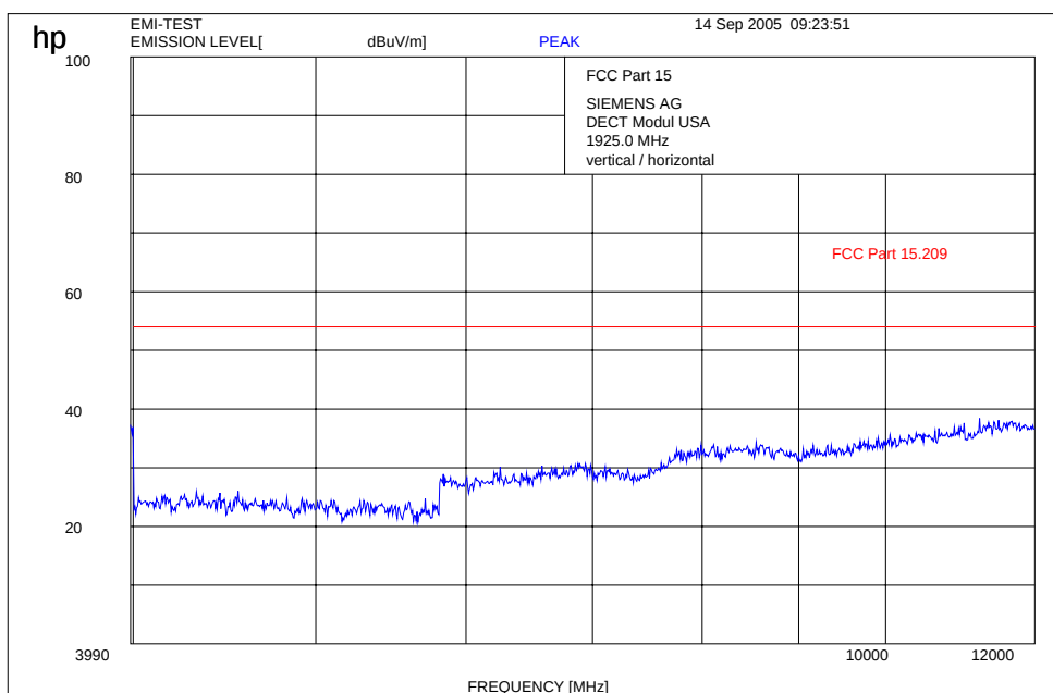
Plot 6: 4 GHz – 12 GHz Transmitter radiated (1925 MHz)
