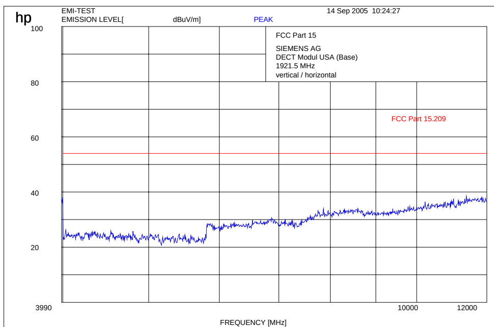
Plot 3: 4 GHz – 12 GHz Transmitter radiated (1921.5 MHz)
