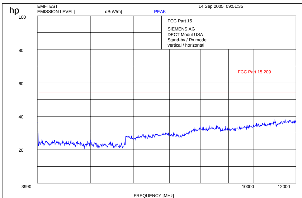
Plot 3: 4 GHz – 12 GHz Receiver radiated (RX / Stand-by Mode)
