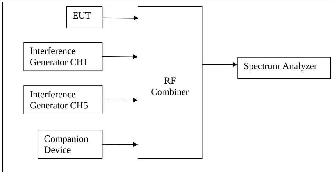
Figure 20: Test Setup for LIC Measurement of VU
