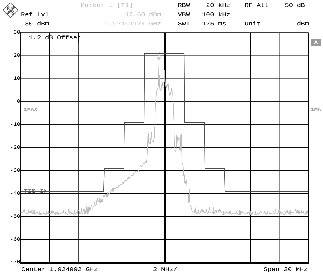
Figure 11: In-Band Spurious Emission of VU at CH3
