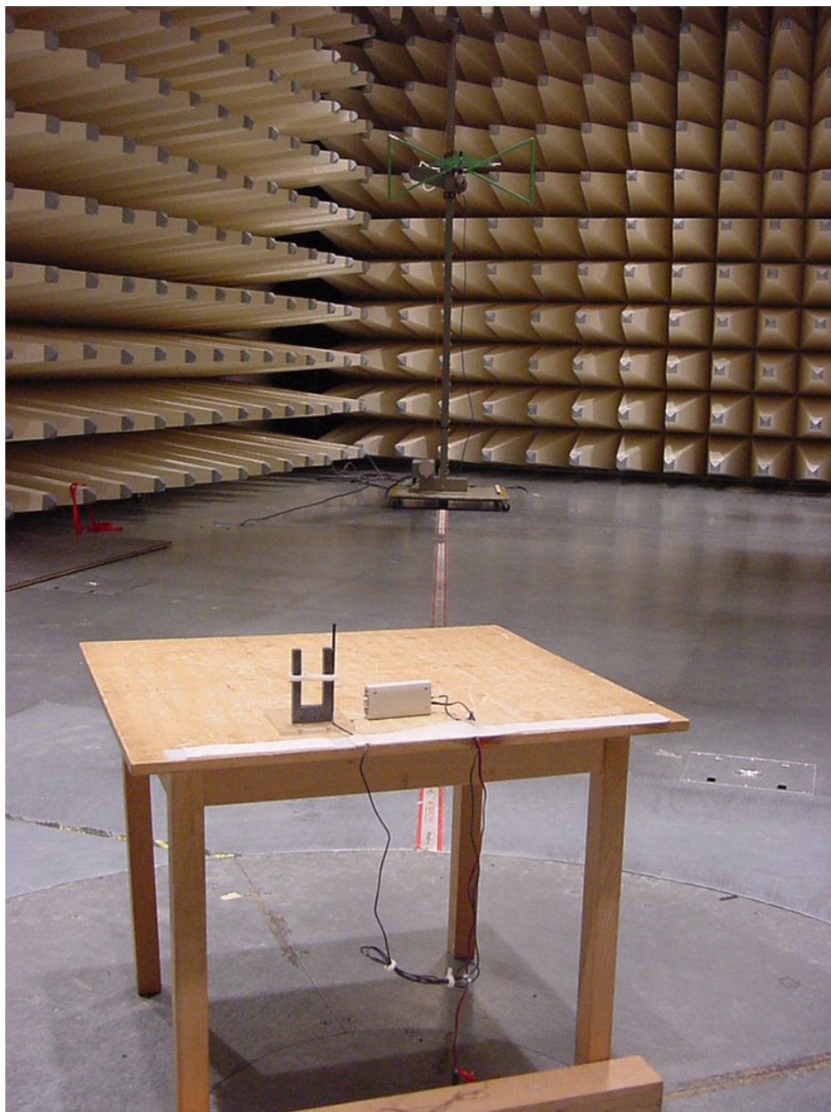
Photo 3 (Radiated Emissions):
