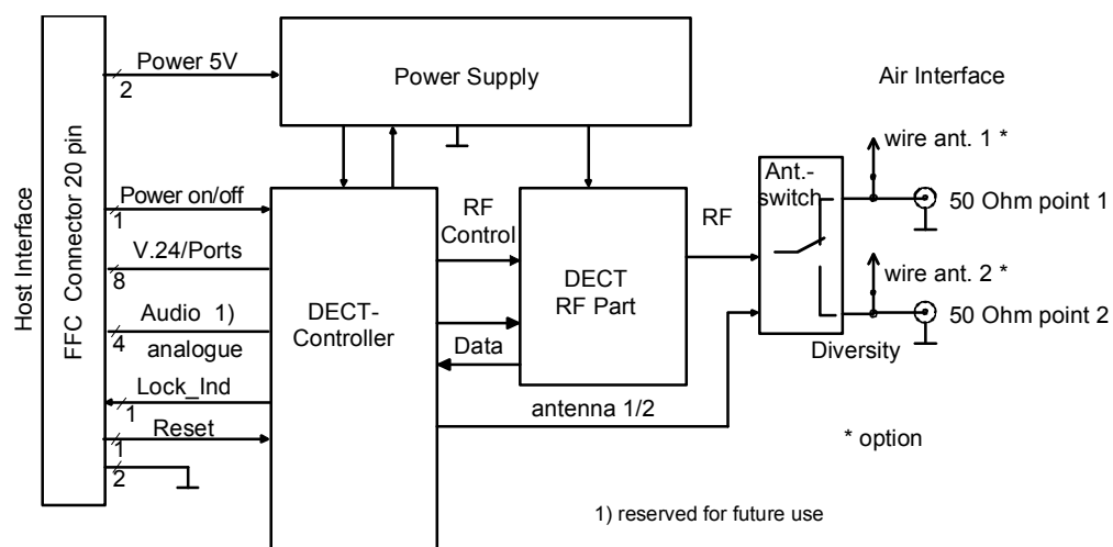
Fig. 2-2 Block Diagram of the DECT Engine
