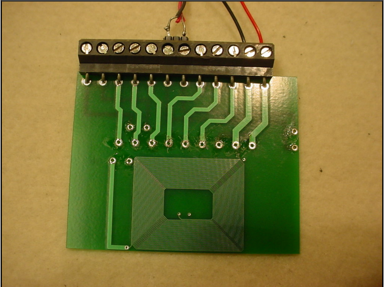
Figure 6: Model 510 Configuration - Magnetic Interface Daughter Board
