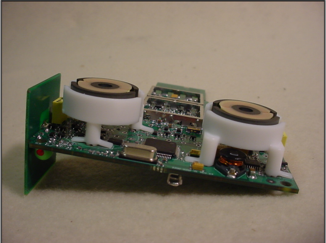
Figure 4: Model 520 Configuration - RF Board w/ Magnetic Interfaces
