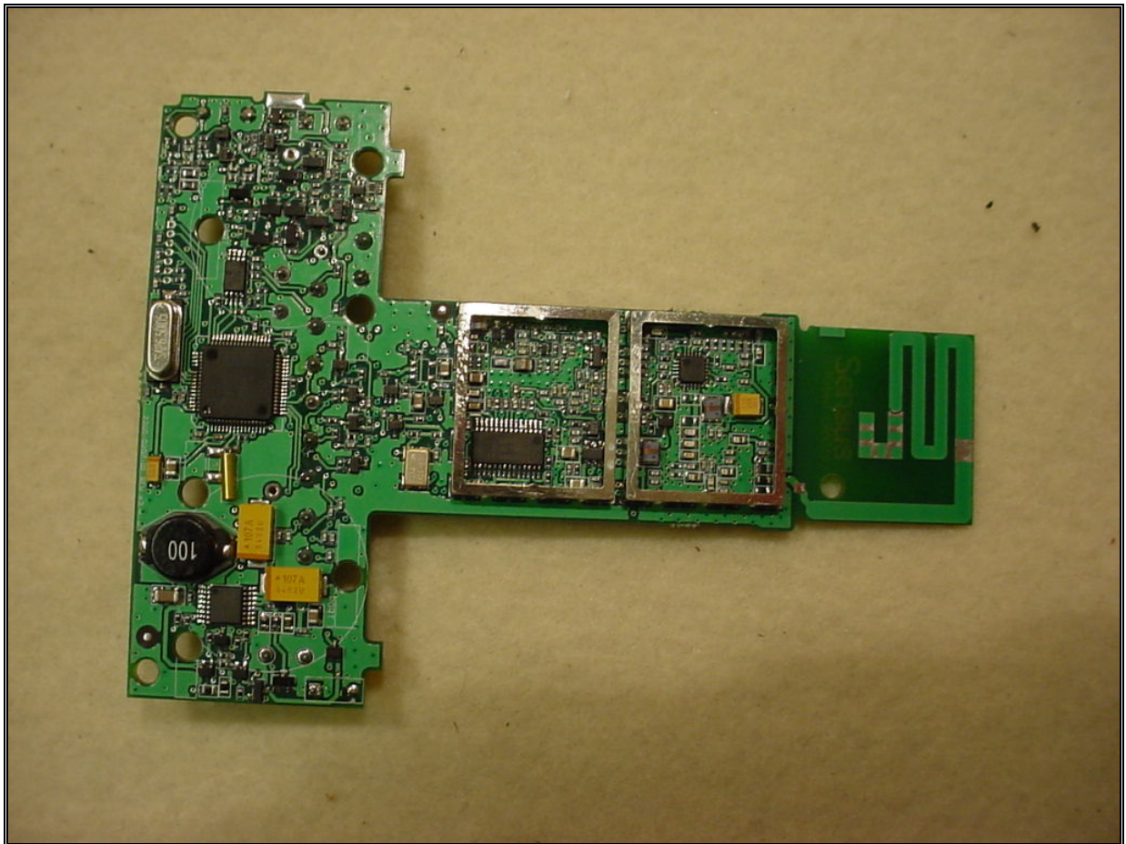
Figure 1: RF Board
