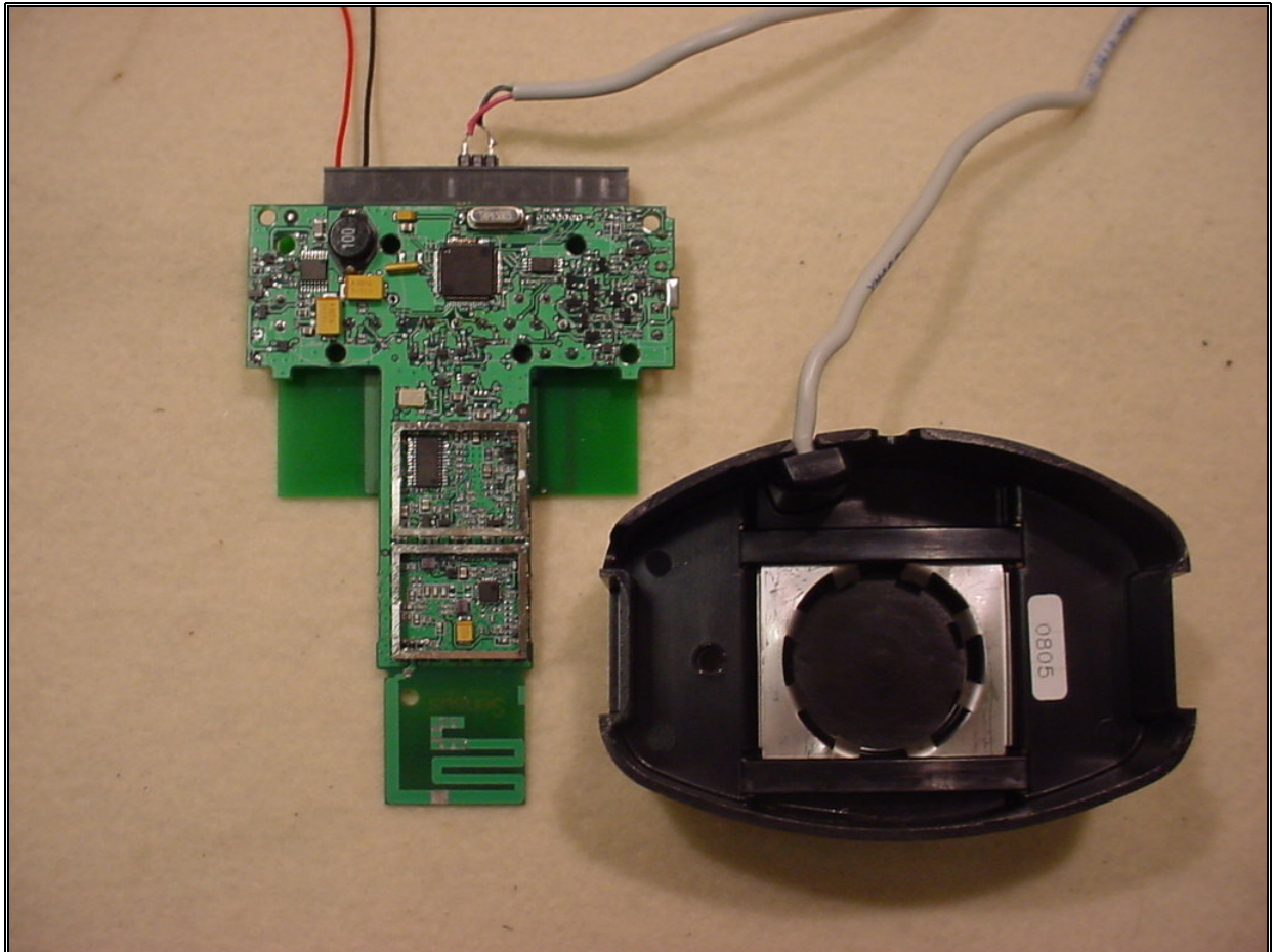
Figure 5: Model 510 Configuration - RF Board w/ Magnetic Interfaces
