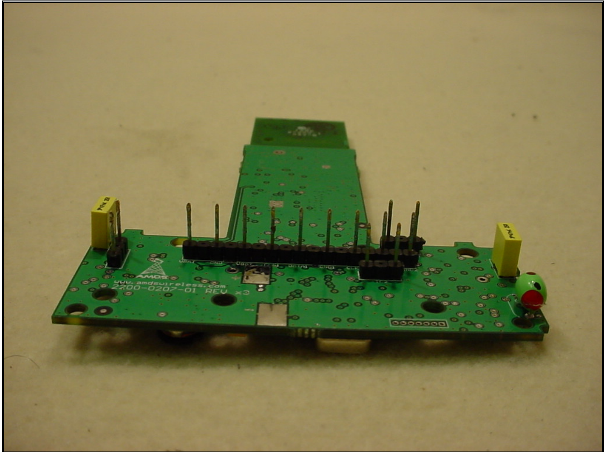
Figure 6: Model 510 Configuration - RF Board w/ Magnetic Interface Daughter Board Removed
