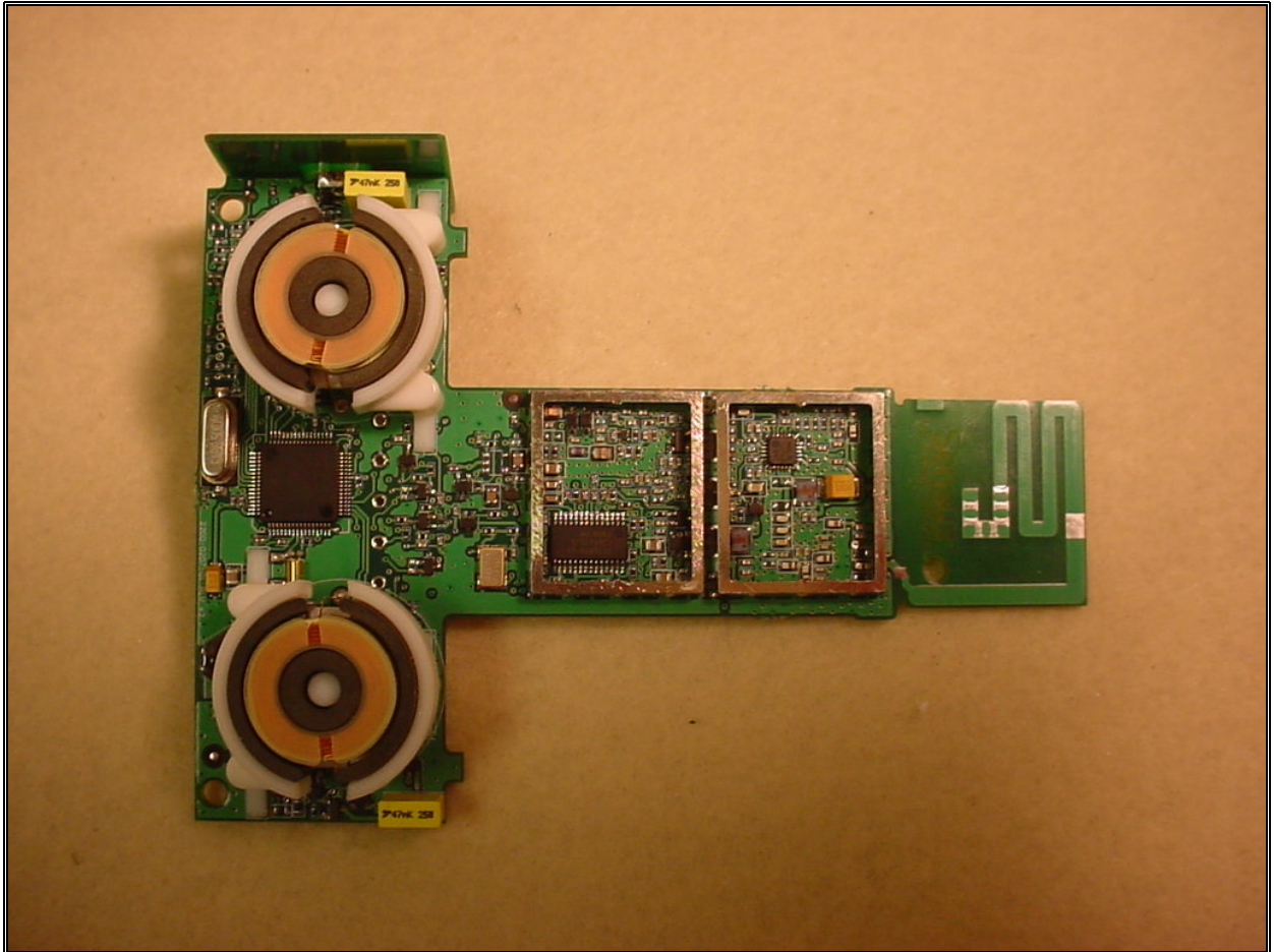
Figure 3: Model 520 Configuration - RF Board w/ Magnetic Interfaces
