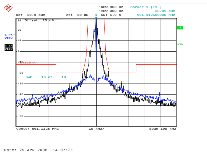
Figure 7.2.2-4: Half-Baud Rate – 901.1125 MHz – 12.5 kHz Channel
