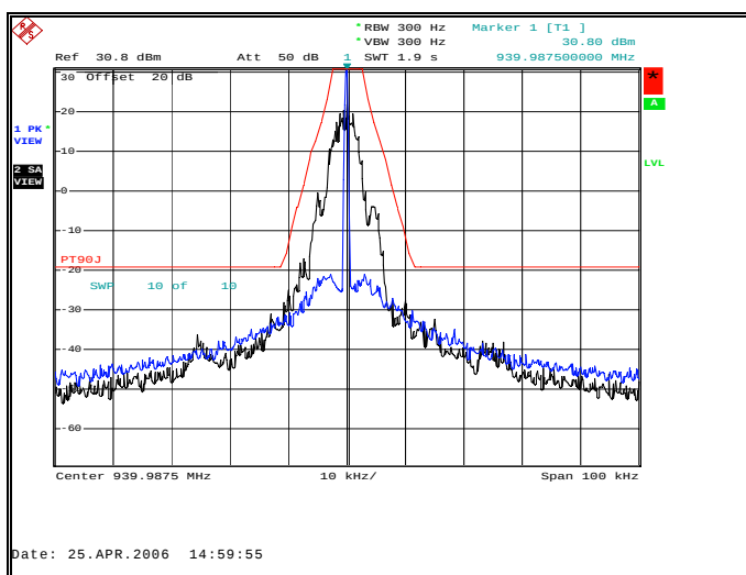
Figure 7.2.3-8: MPass Mode – 939.9875 MHz
