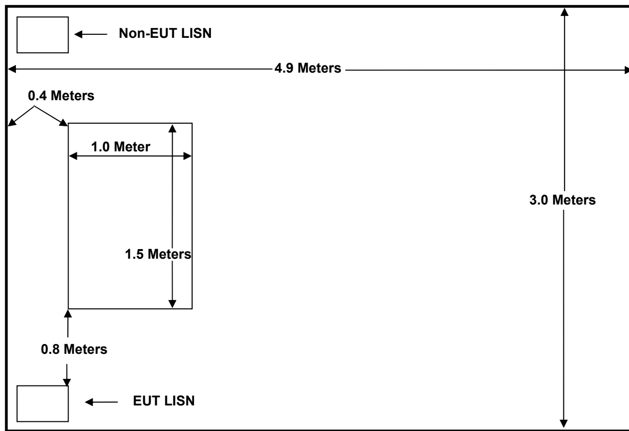
Figure 2.1.2-1: AC Mains Conducted EMI Site
