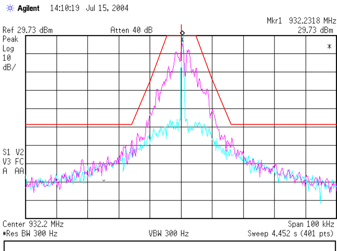
Figure 7.2.2-1: Normal Mode – 932.23125 MHz
