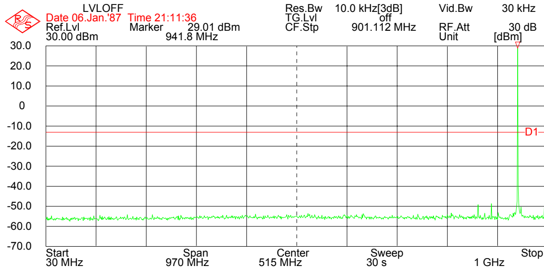
Figure 7.3.2-3: Normal Mode -941.23125 MHz
