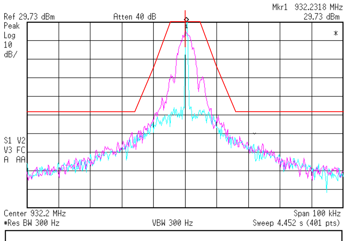
Figure 7.2.2-2: Mpass Mode – 932.23125 MHz
