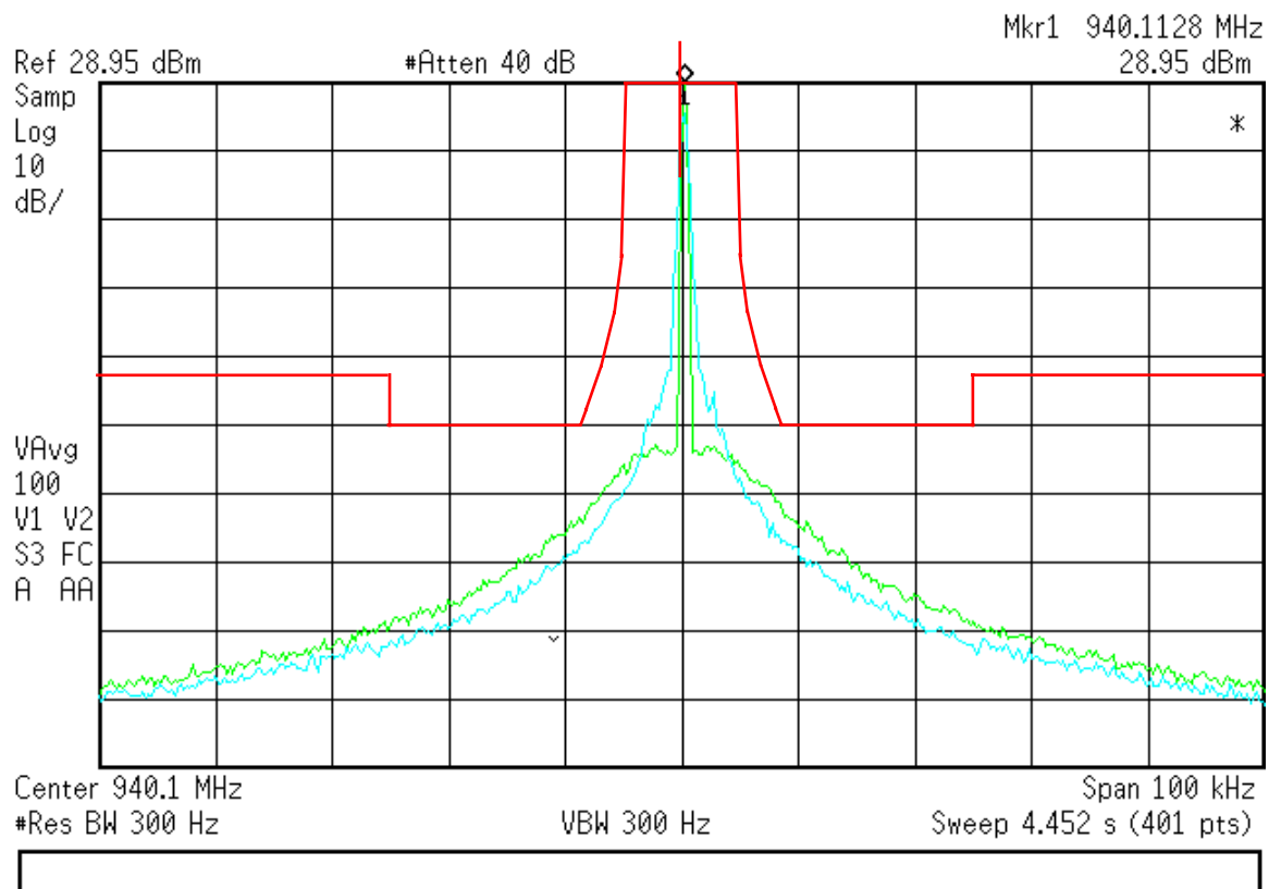
Figure 7.2.2-11: Boost Mode – 940.1125 MHz – 12.5 kHz Channel
