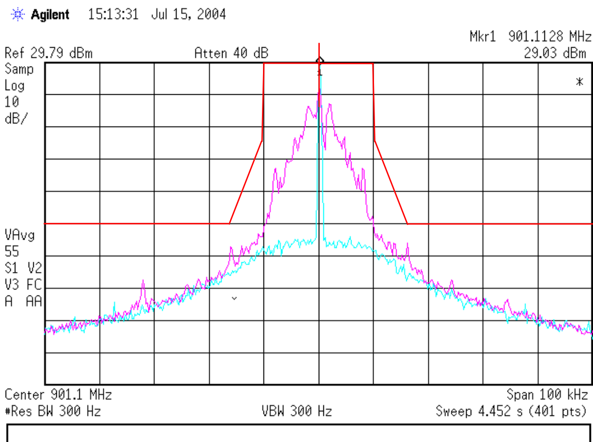
Figure 7.2.2-1: Normal Mode – 901.1125 MHz – 25 kHz Channel
