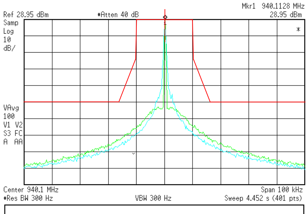
Figure 7.2.2-10: Boost Mode – 940.1125 MHz – 25 kHz Channel
