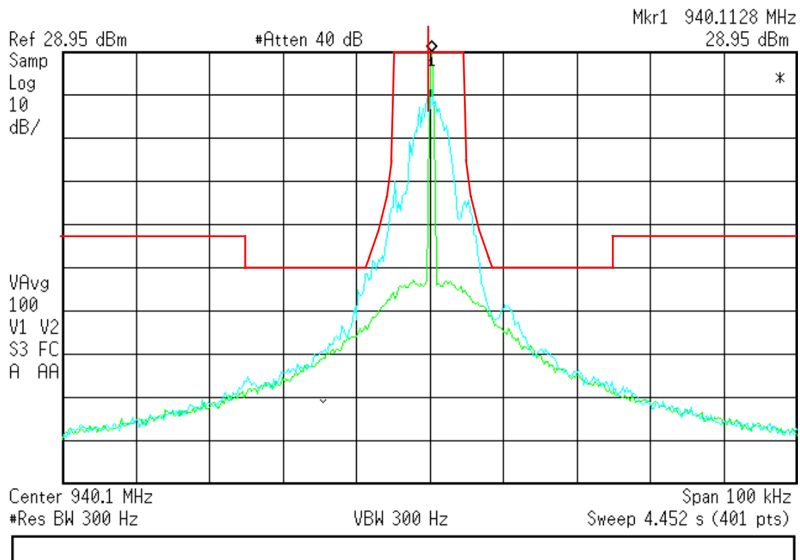
Figure 7.2.2-9: MPass Mode – 940.1125 MHz – 12.5 kHz Channel
