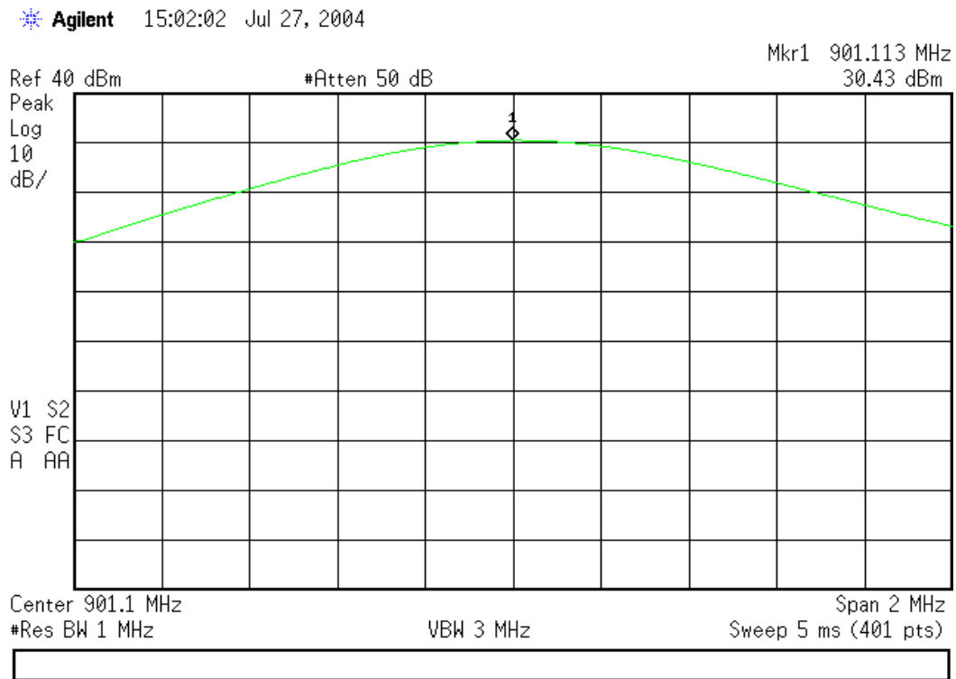
Figure 7.1.2-1: Peak Output Power 901.1125 MHz
