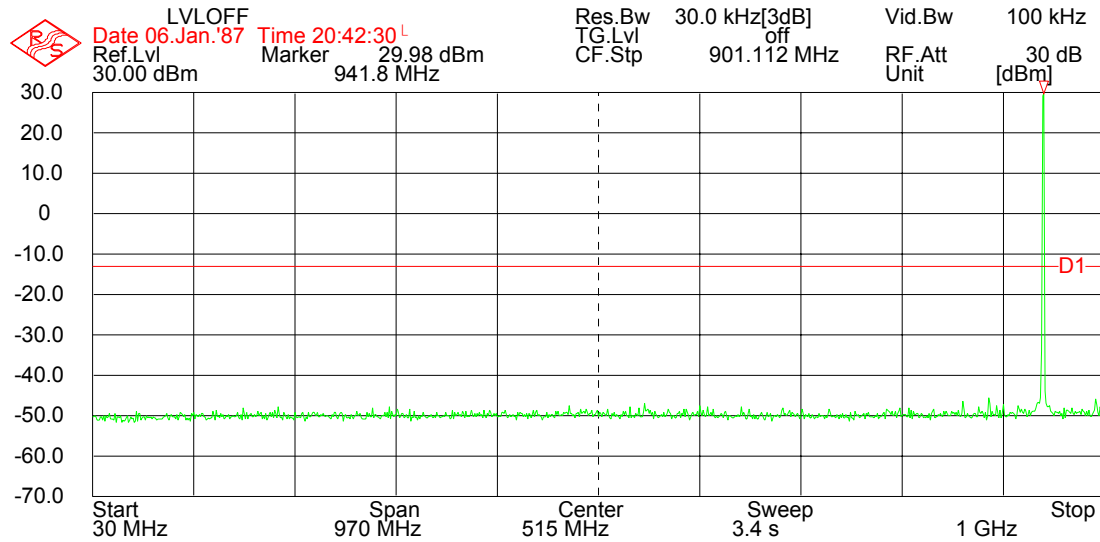
Figure 7.3.2-3: Normal Mode -940.1125 MHz
