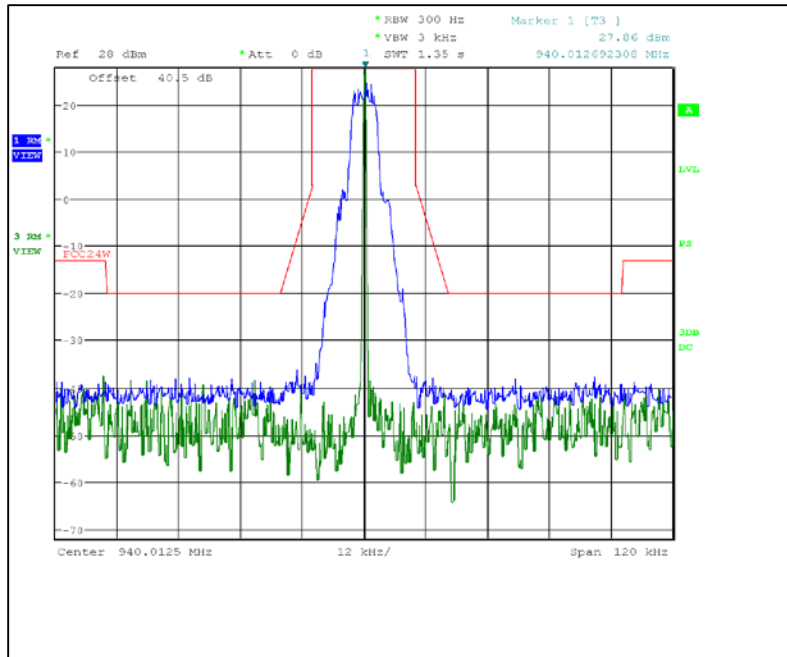
Figure 7.2.2-11: 940.0125 MHz – 25 kHz Channel Spacing – mPass 5k Mode
