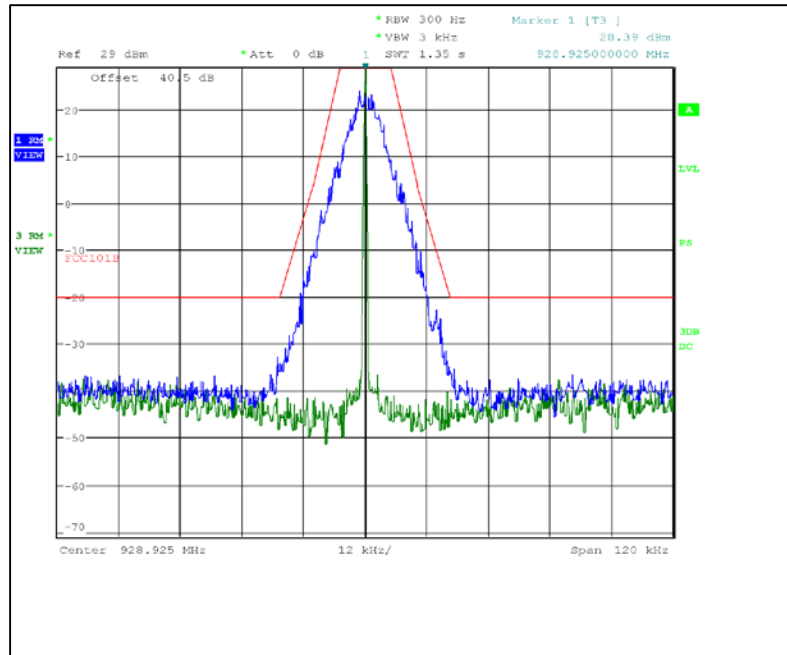
Figure 7.2.2-15: 928.925 MHz – Double Density Mode
