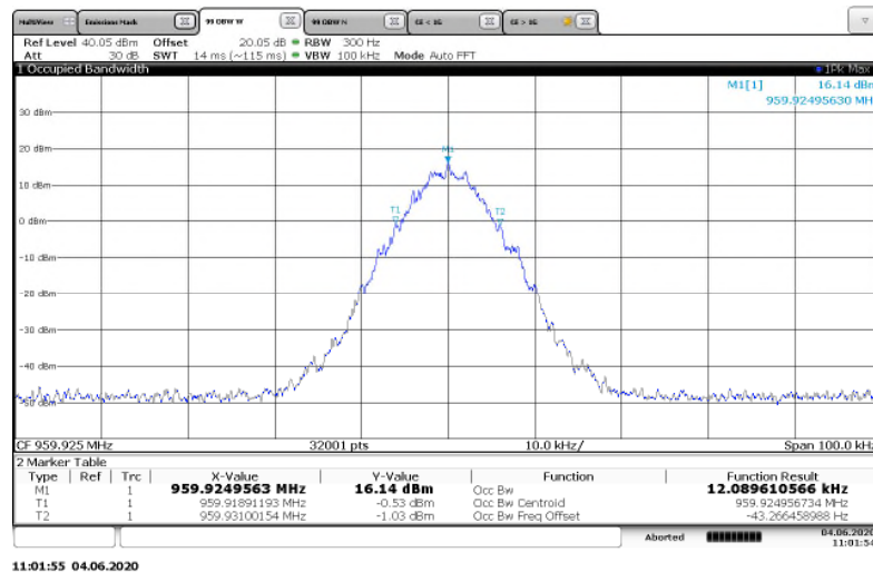
Figure 7.3.2-31: 959.925 MHz – MPass 12.5k Mode
