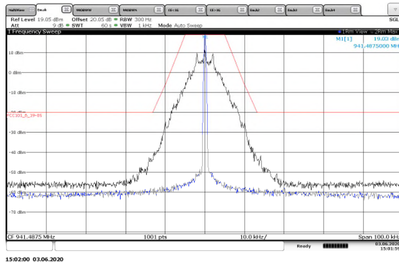
Figure 7.2.2-25: 941.4875 MHz – 25 kHz Channel Spacing – mPass 12.5k Mode
