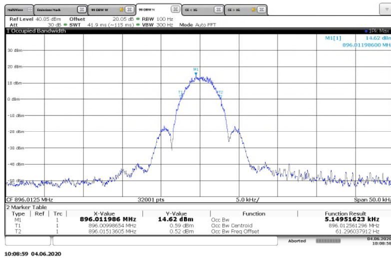
Figure 7.3.2-9: 896.0125 MHz – MPass 5k Mode
