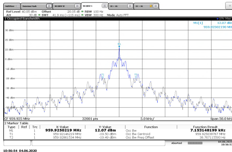
Figure 7.3.2-32: 959.925 MHz – ASK Mode
