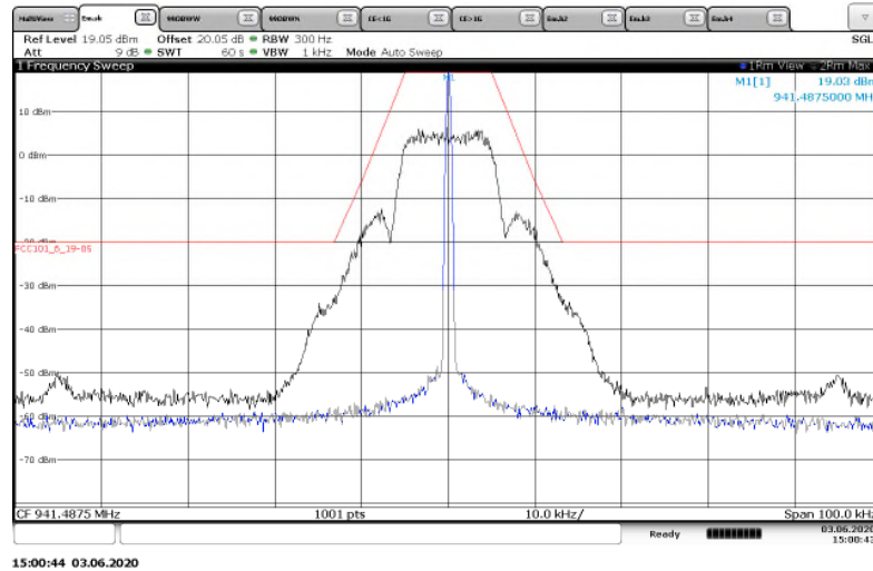
Figure 7.2.2-24: 941.4875 MHz – 25 kHz Channel Spacing – mPass 10k Mode
