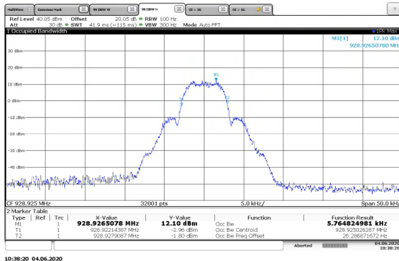
Figure 7.3.2-11: 928.925 MHz – MPass 5k Mode
