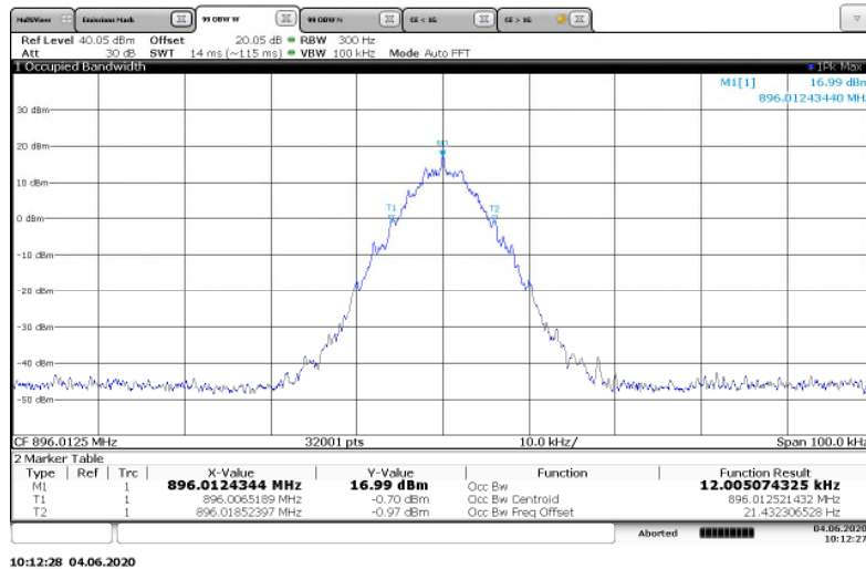
Figure 7.3.2-10: 896.0125 MHz – MPass 12.5k Mode
