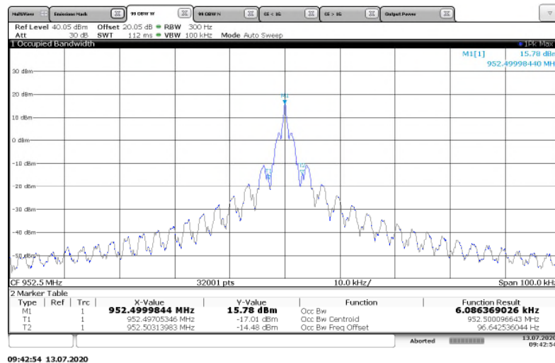
Figure 7.3.2-28: 952.5 MHz – ASK Mode
