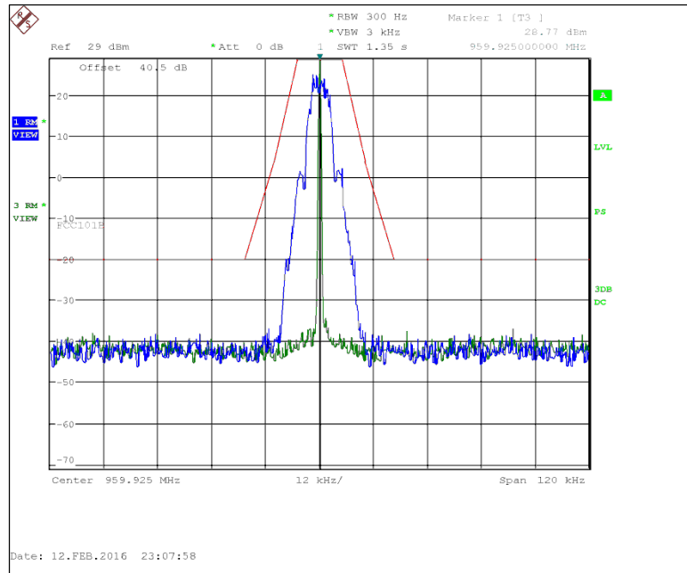
Figure 7.2.2-25: 959.925 MHz – mPass 5k Mode
