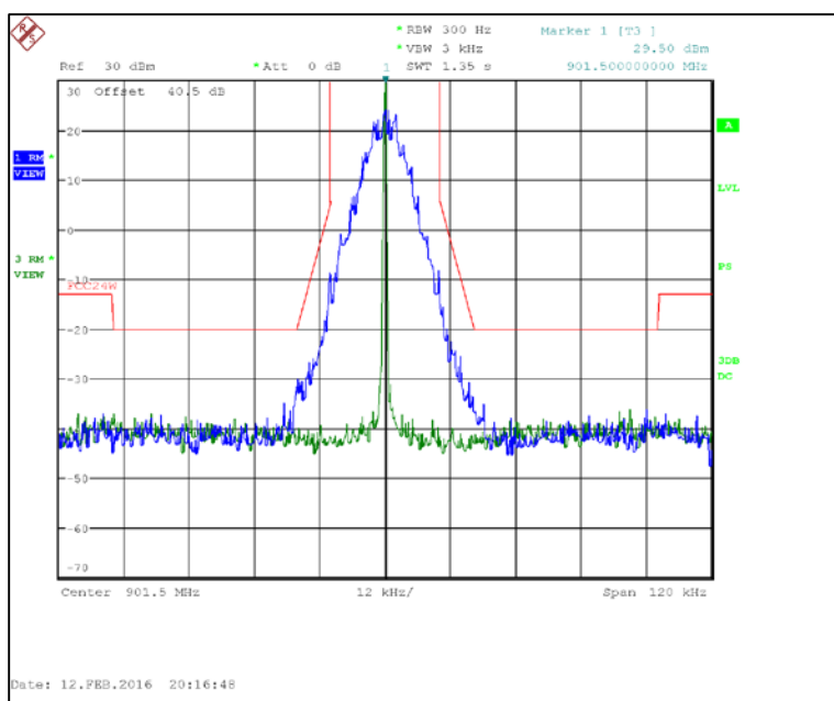
Figure 7.2.2-2: 901.5 MHz – 25 kHz Channel Spacing – Normal Mode
