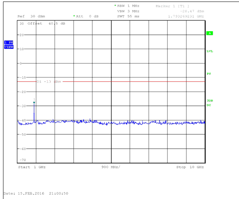
Figure 7.3.2-2: 901.5 MHz – 1GHz to 10GHz
