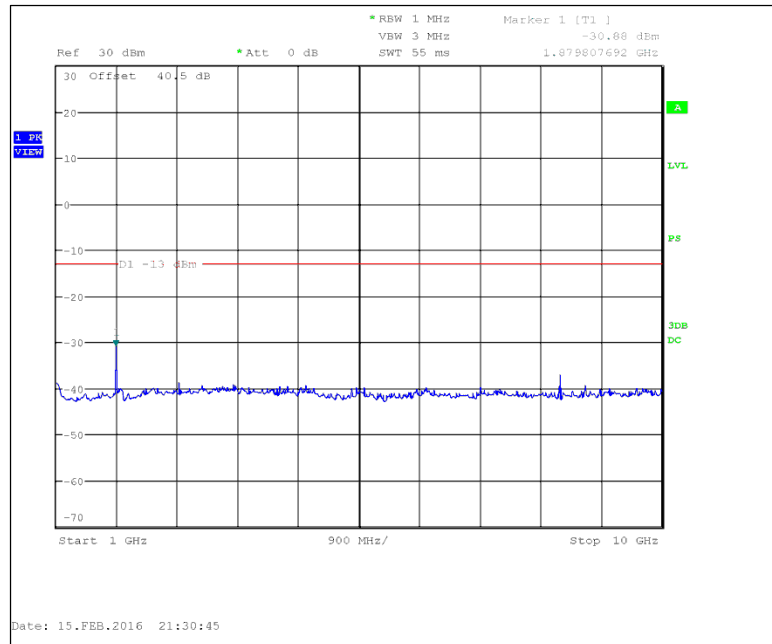
Figure 7.3.2-12: 941.4875 MHz – 1GHz to 10GHz
