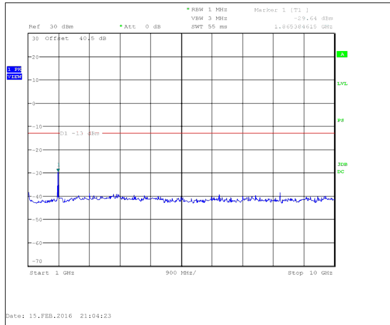
Figure 7.3.2-10: 932.25 MHz – 1GHz to 10GHz
