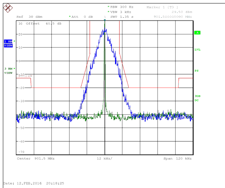
Figure 7.2.2-6: 901.5 MHz – 25 kHz Channel Spacing – Double Density Mode
