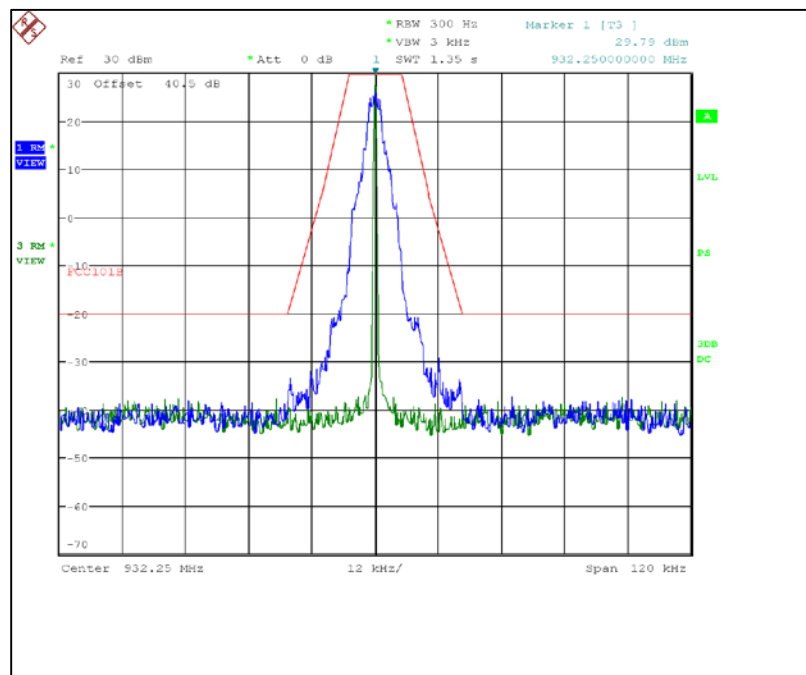
Figure 7.2.2-18: 932.25 MHz – C&amp;I Mode
