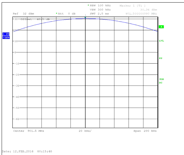
Figure 7.1.2-1: 901.5 MHz
