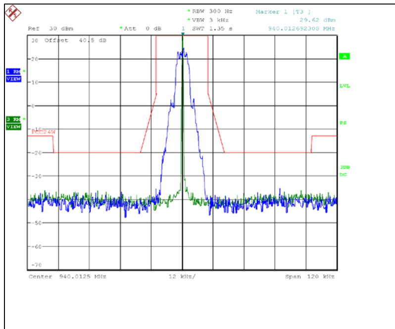
Figure 7.2.2-11: 940.0125 MHz – 25 kHz Channel Spacing – mPass 5k Mode
