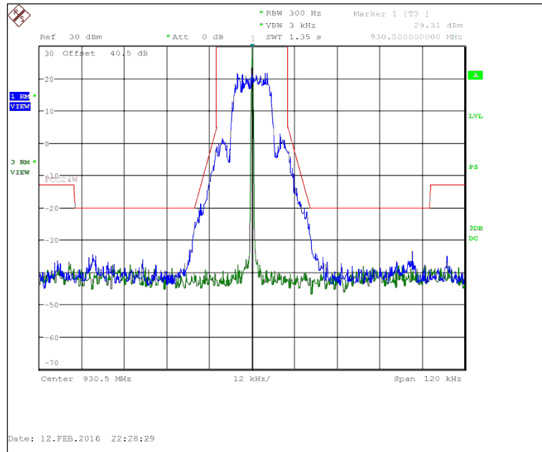
Figure 7.2.2-9: 930.5 MHz – 25 kHz Channel Spacing – mPass 10k Mode
