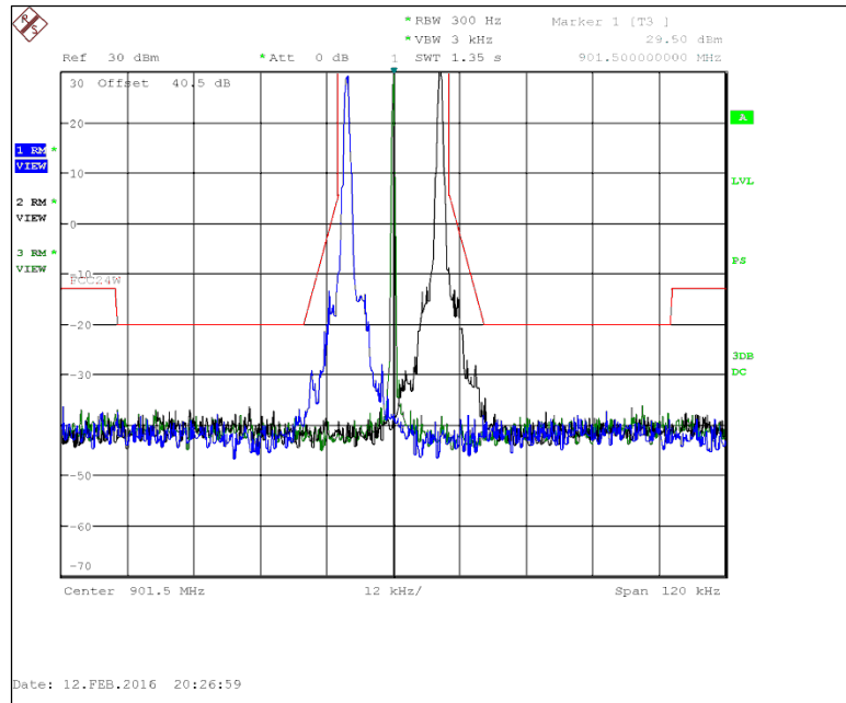
Figure 7.2.2-3: 901.5 MHz – 25 kHz Channel Spacing – Boost Mode
