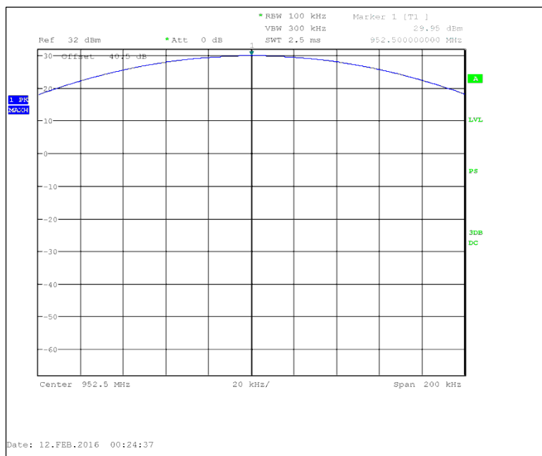
Figure 7.1.2-7: 952.5 MHz
