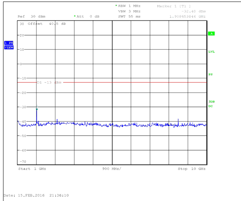
Figure 7.3.2-16: 959.925 MHz – 1GHz to 10GHz
