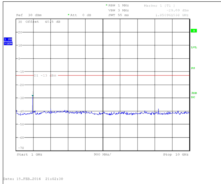
Figure 7.3.2-4: 930.5 MHz – 1GHz to 10GHz
