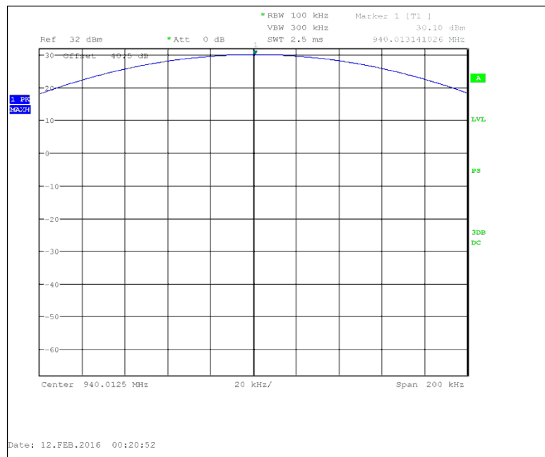
Figure 7.1.2-3: 940.0125 MHz
