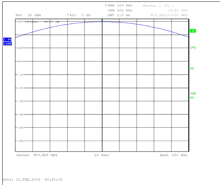
Figure 7.1.2-8: 959.925 MHz
