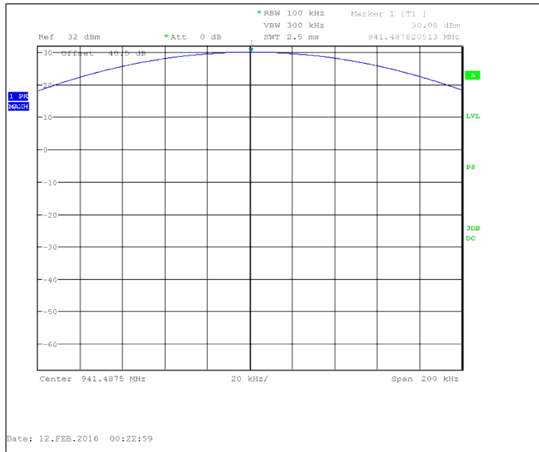
Figure 7.1.2-6: 941.4875 MHz
