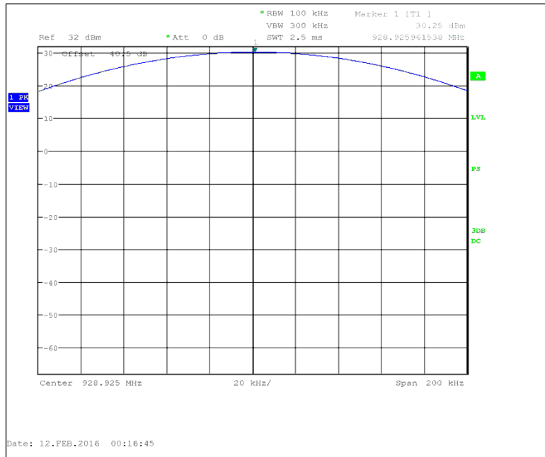
Figure 7.1.2-4: 928.925 MHz
