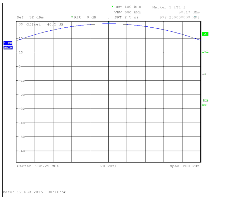
Figure 7.1.2-5: 932.25 MHz
