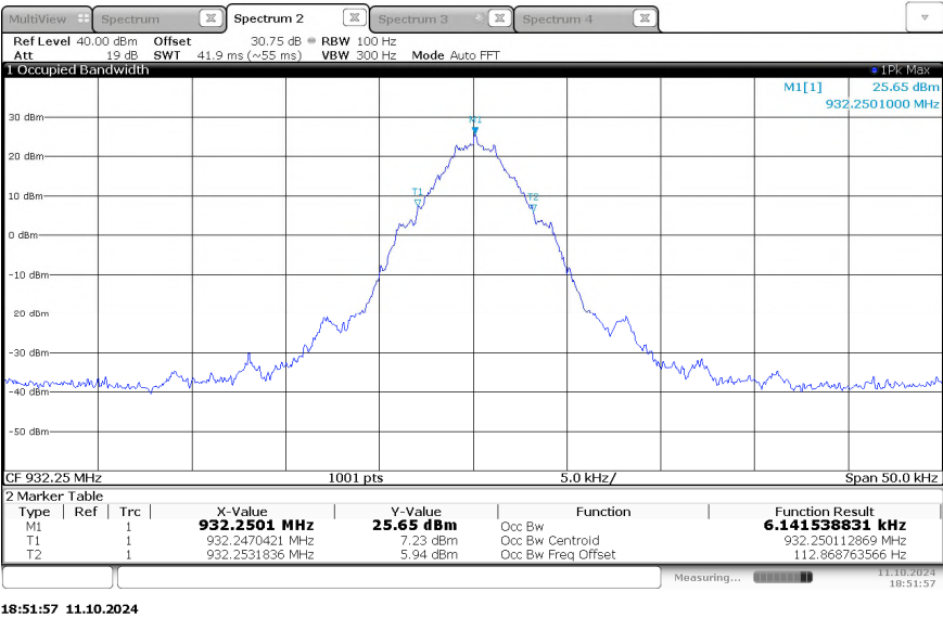
Figure 2.3.6-12 - 99% Bandwidth – TXC TCXO – 932.25 MHz - C&I Mode
