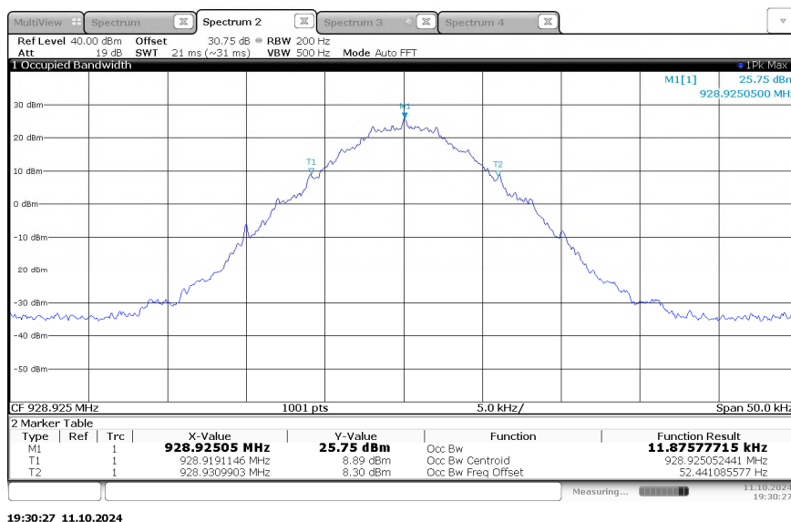
Figure 2.3.6-7 - 99% Bandwidth – TXC TCXO – 928.925 MHz - Normal Mode
