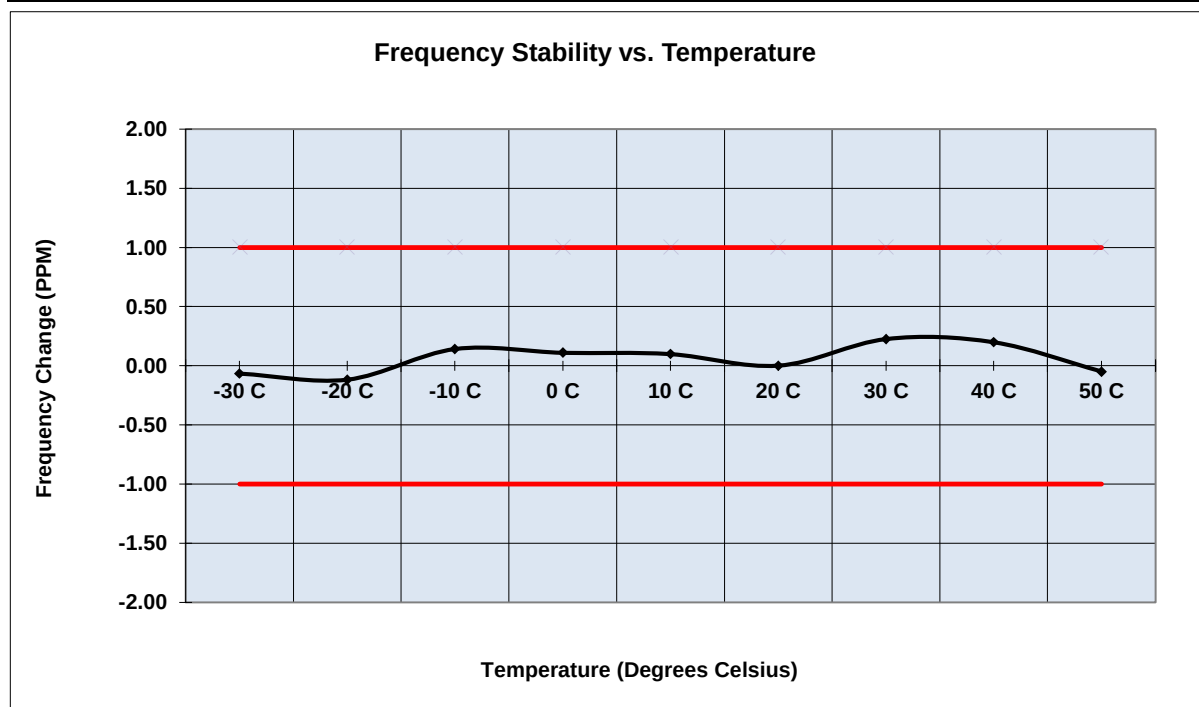
Figure 2.6.6-1 - Frequency Stability – KDS TCXO – 901.5 MHz
