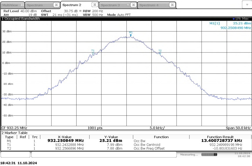
Figure 2.3.6-14 - 99% Bandwidth – TXC TCXO – 932.25 MHz - Double Density Mode
