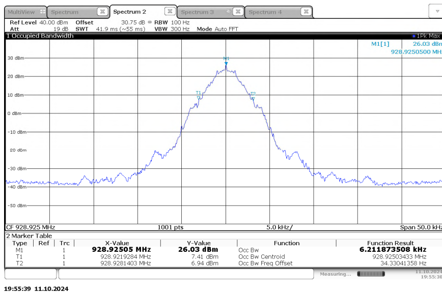
Figure 2.3.6-6 - 99% Bandwidth – TXC TCXO – 928.925 MHz - C&amp;I Mode
