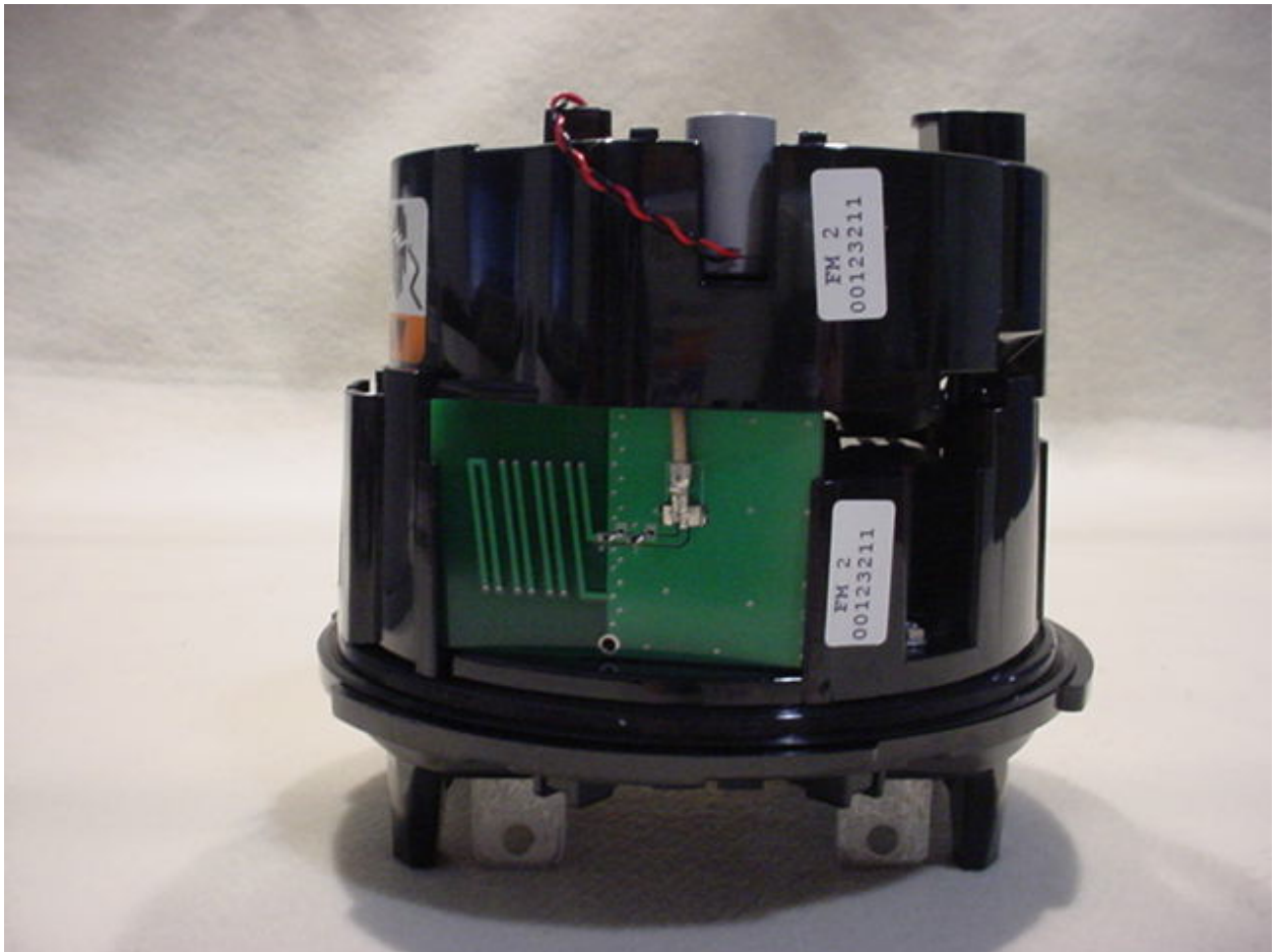
Figure 4: External Photographs – Side View Housing Removed
