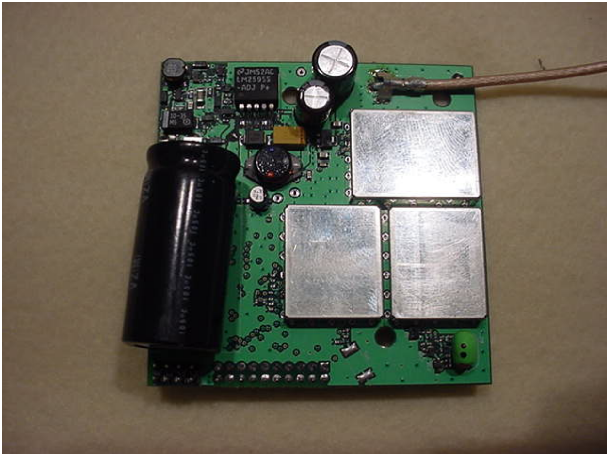
Figure 1: Internal Photographs – Top View RF PCB
