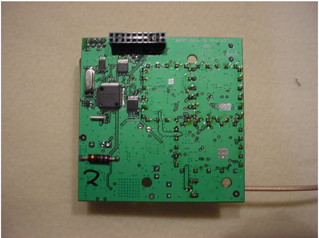
Figure 3: Internal Photographs – Bottom View RF PCB
