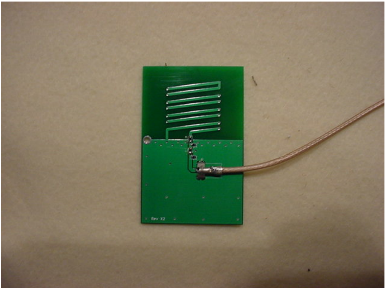
Figure 4: Internal Photographs – Top View Antenna
