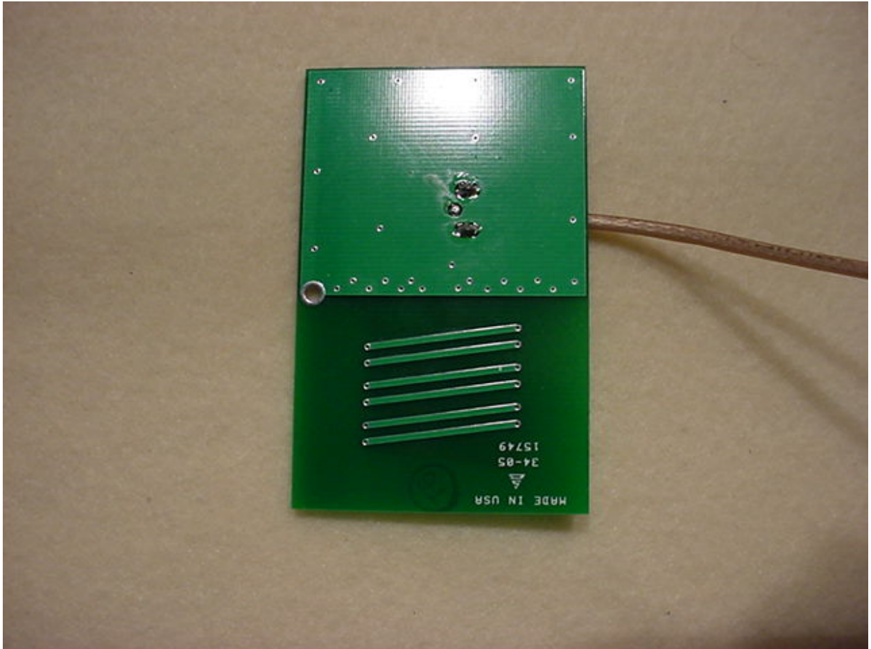
Figure 5: Internal Photographs – Bottom View Antenna
