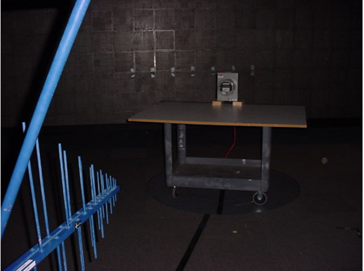
Figure 4: Radiated Emissions – Unintentional – 120VAC Front View
