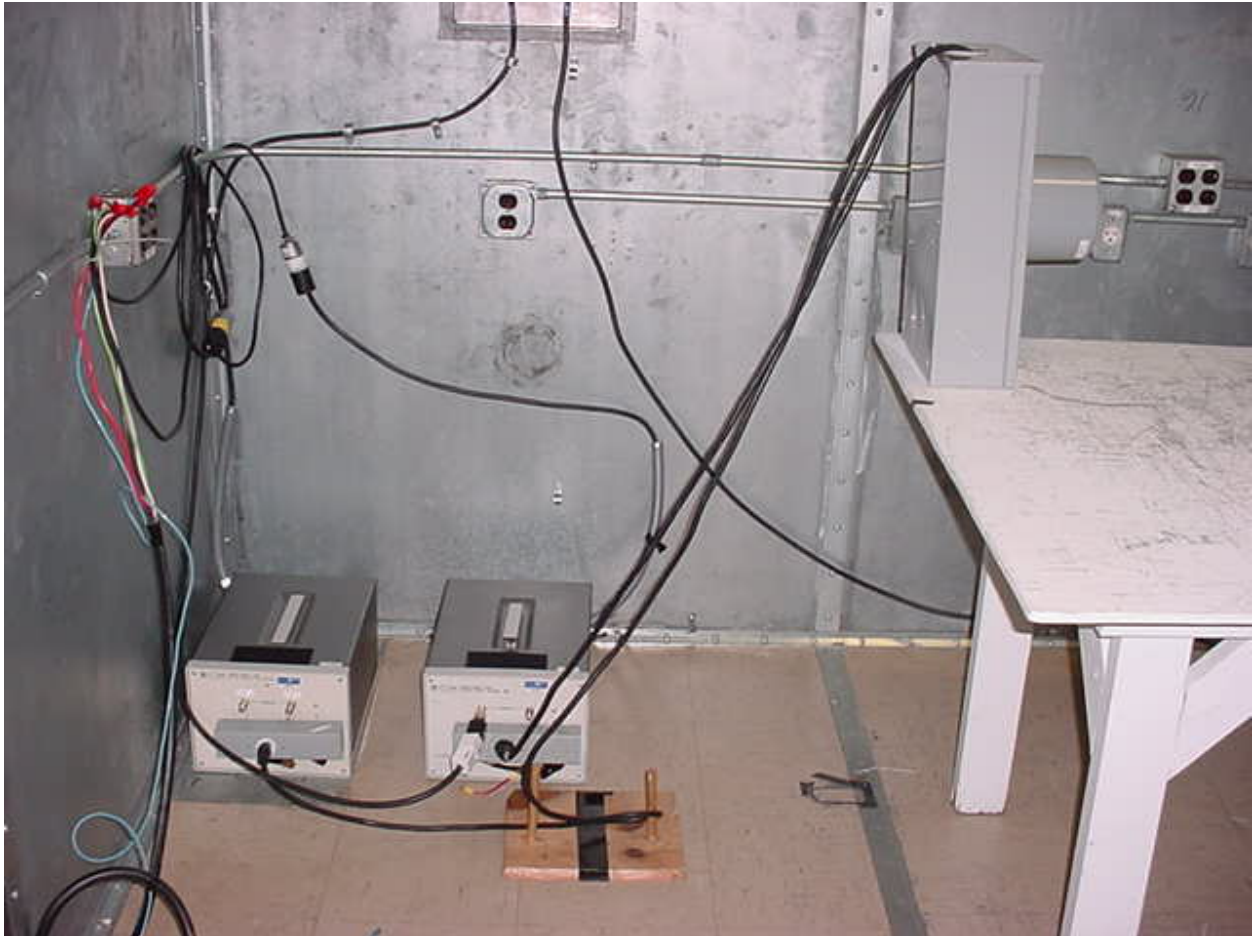
Figure 8: Conducted Emissions – Unintentional – 240 VAC
