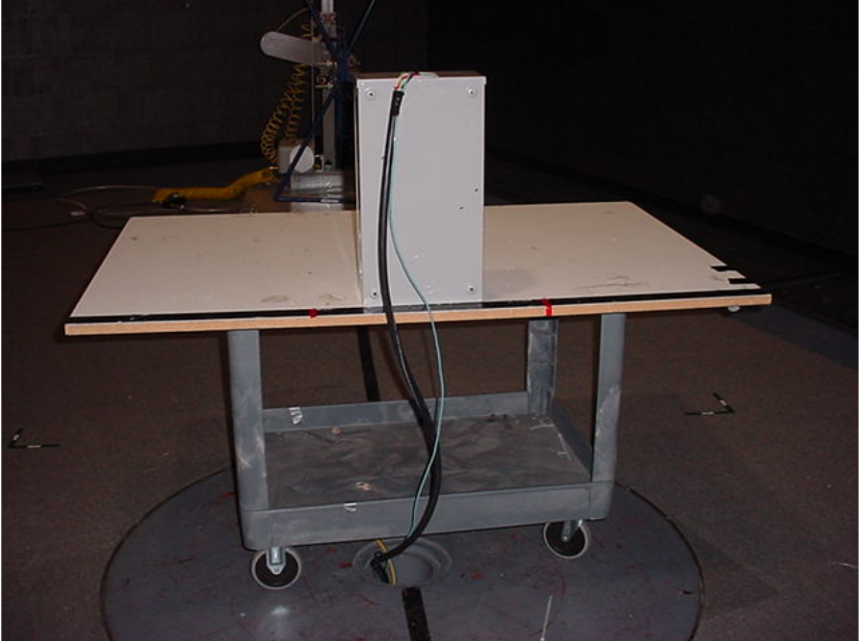
Figure 5: Radiated Emissions – Unintentional – 240 VAC Rear View
