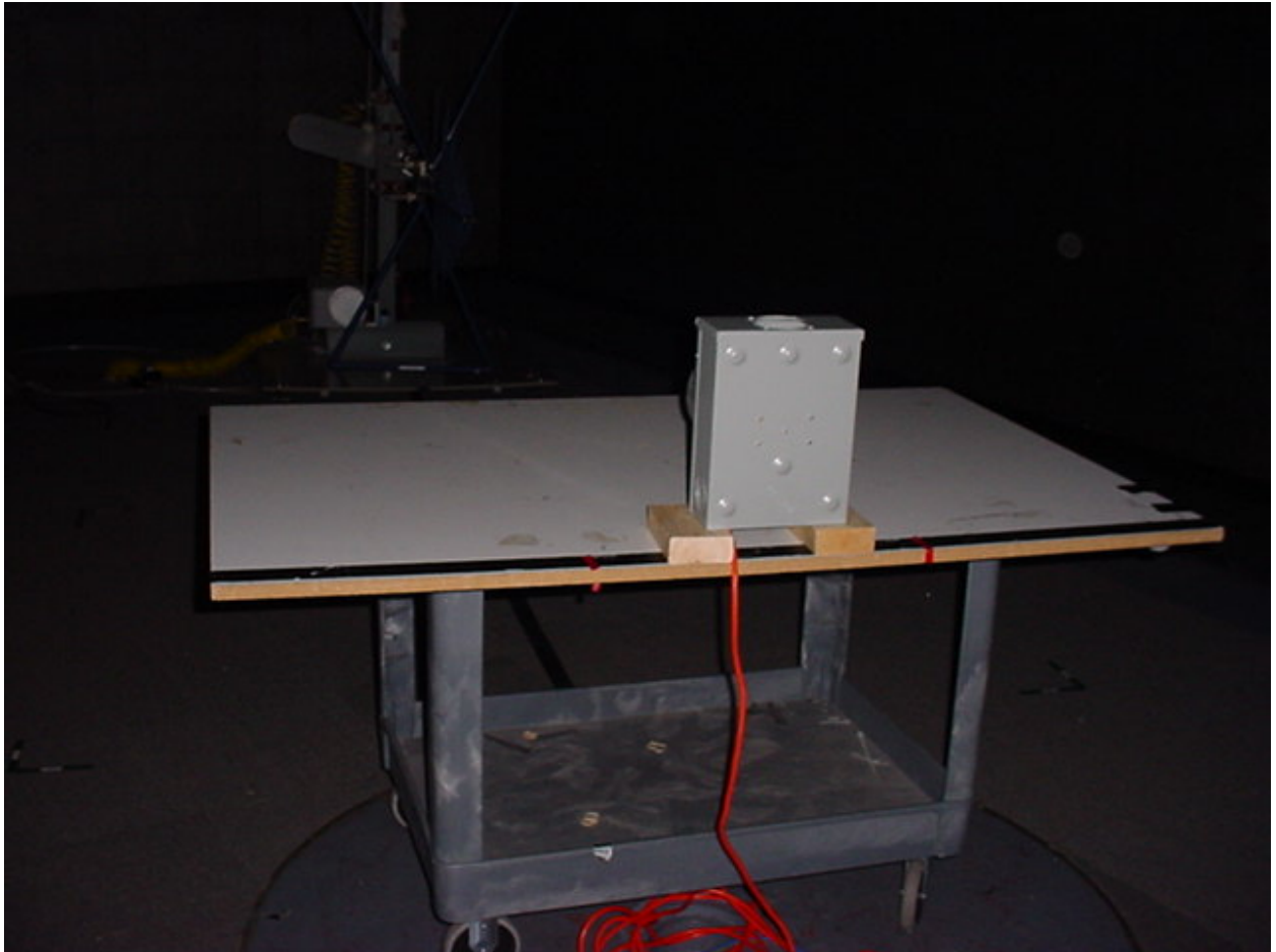
Figure 3: Radiated Emissions – Unintentional – 120VAC Rear View
