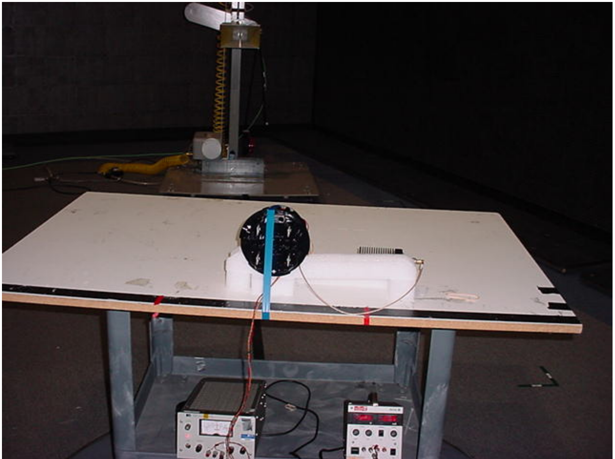
Figure 1: Radiated Emissions – Transmitter Rear View
