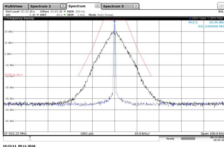
Figure 7.2.2-30: 932.25 MHz – 25 kHz Channel Spacing – Double Density Mode
