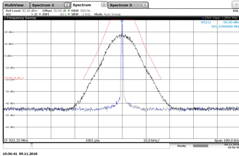
Figure 7.2.2-37: 932.25 MHz – 25 kHz Channel Spacing – 4FSK Mode
