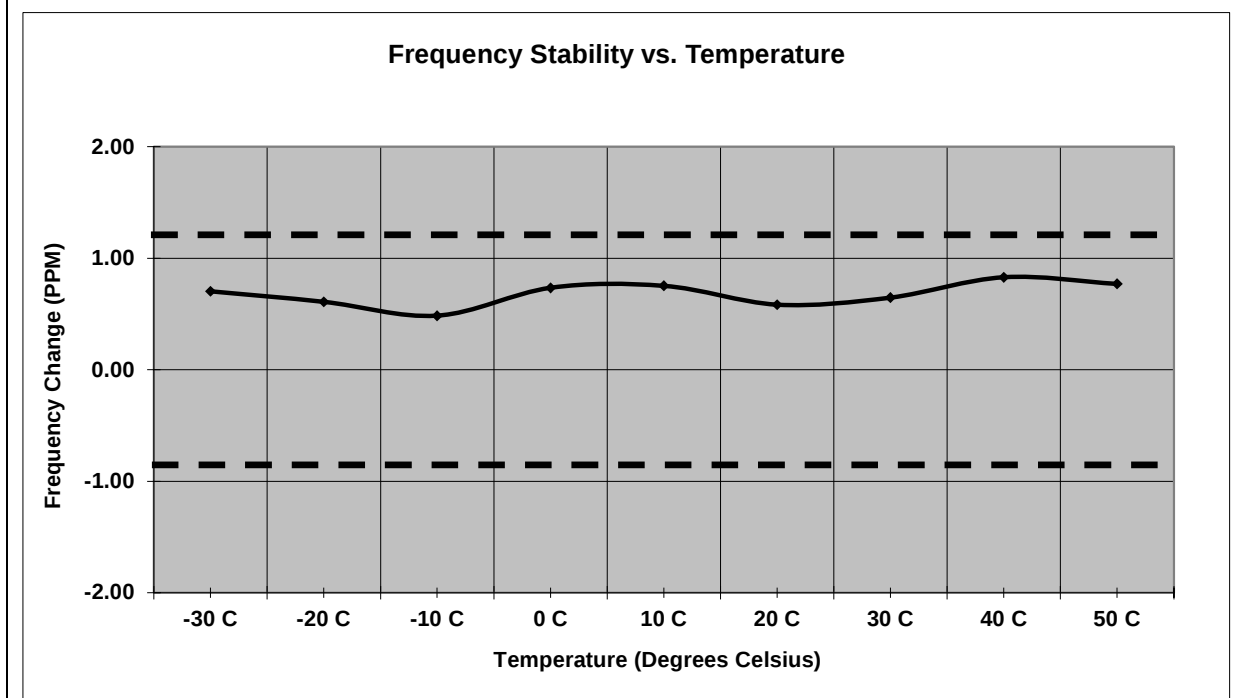
Figure 7.6.2-5: Frequency Stability – 930.5 MHz – TXC
