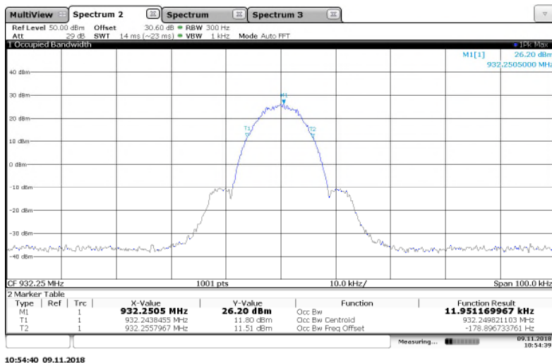
Figure 7.3.2-36: 932.25 MHz – 2FSK Mode
