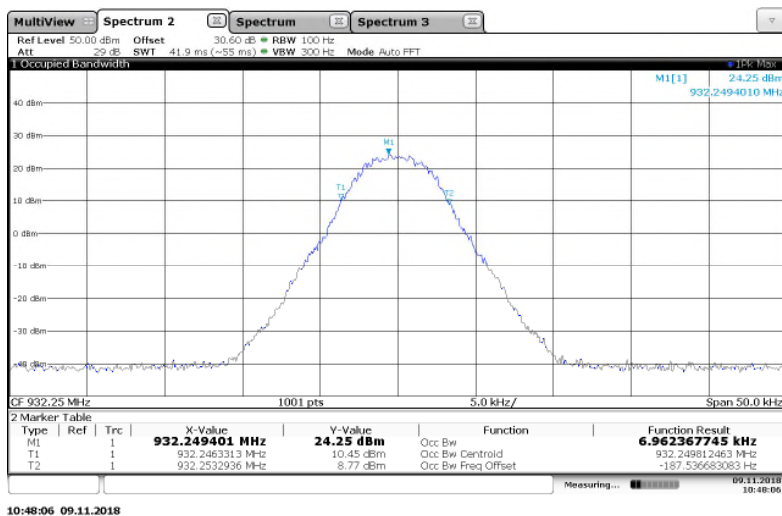
Figure 7.3.2-34: 932.25 MHz – 4FSK (Half Baud) Mode
