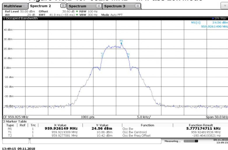
Figure 7.3.2-47: 959.925 MHz – MPass 5k Mode
