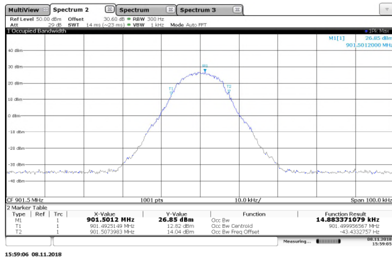
Figure 7.3.2-10: 901.5 MHz – 8FSK Mode
