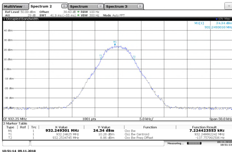
Figure 7.3.2-35: 932.25 MHz – 8FSK (Half Baud) Mode
