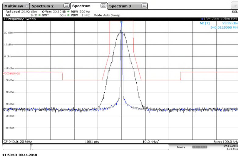
Figure 7.2.2-17: 940.0125 MHz – 25 kHz Channel Spacing – m4Pass 10k Mode
