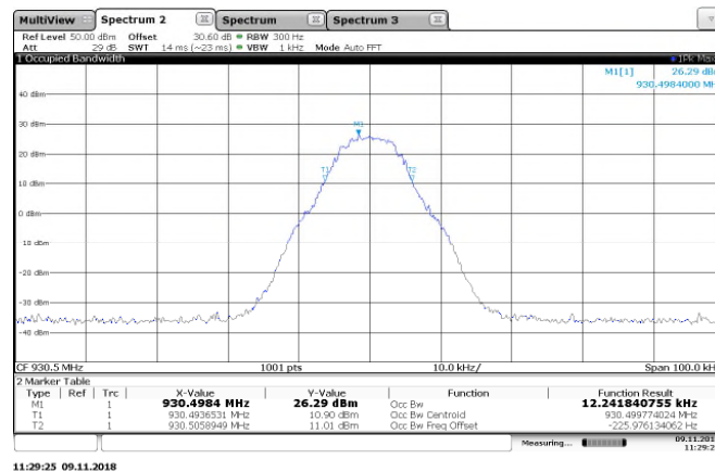
Figure 7.3.2-14: 930.5 MHz – M4Pass 20k Mode
