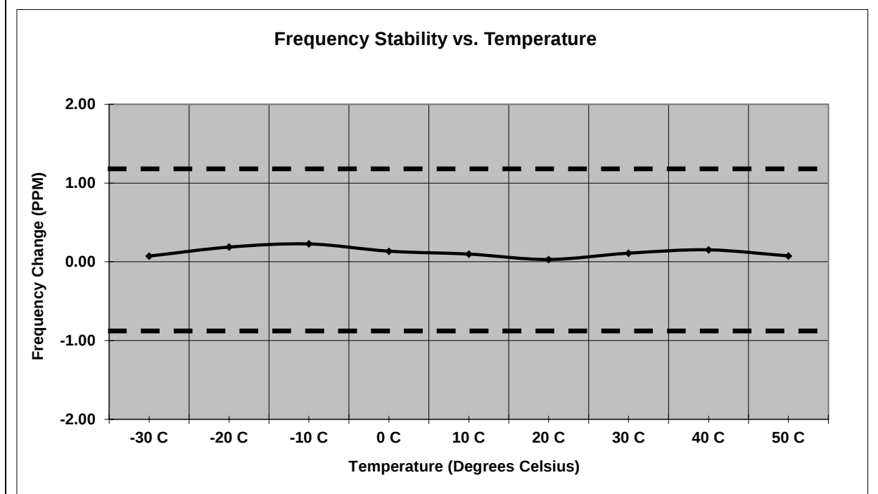
Figure 7.6.2-4: Frequency Stability – 930.5 MHz – KDS
