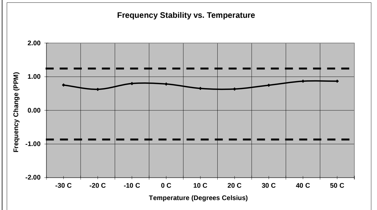
Figure 7.6.2-2: Frequency Stability – 901.5 MHz – TXC
