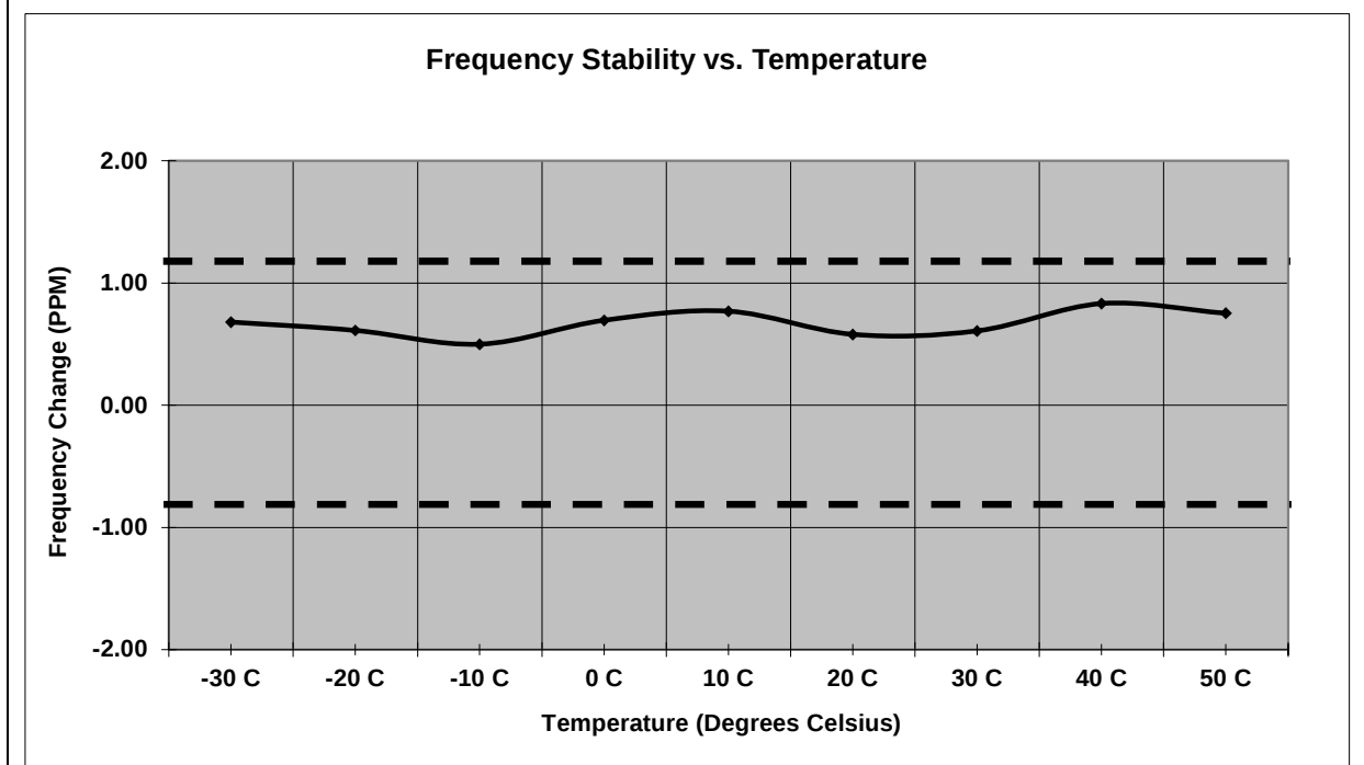
Figure 7.6.2-8: Frequency Stability – 959.925 MHz – TXC
