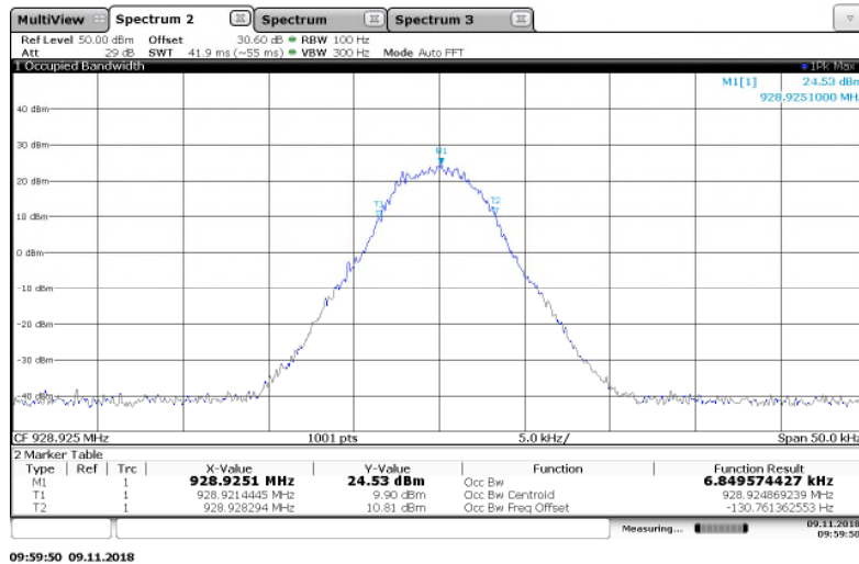
Figure 7.3.2-24: 928.925 MHz – 4FSK (Half Baud) Mode
