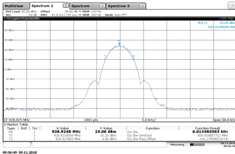
Figure 7.3.2-23: 928.925 MHz – 2FSK (Half Baud) Mode
